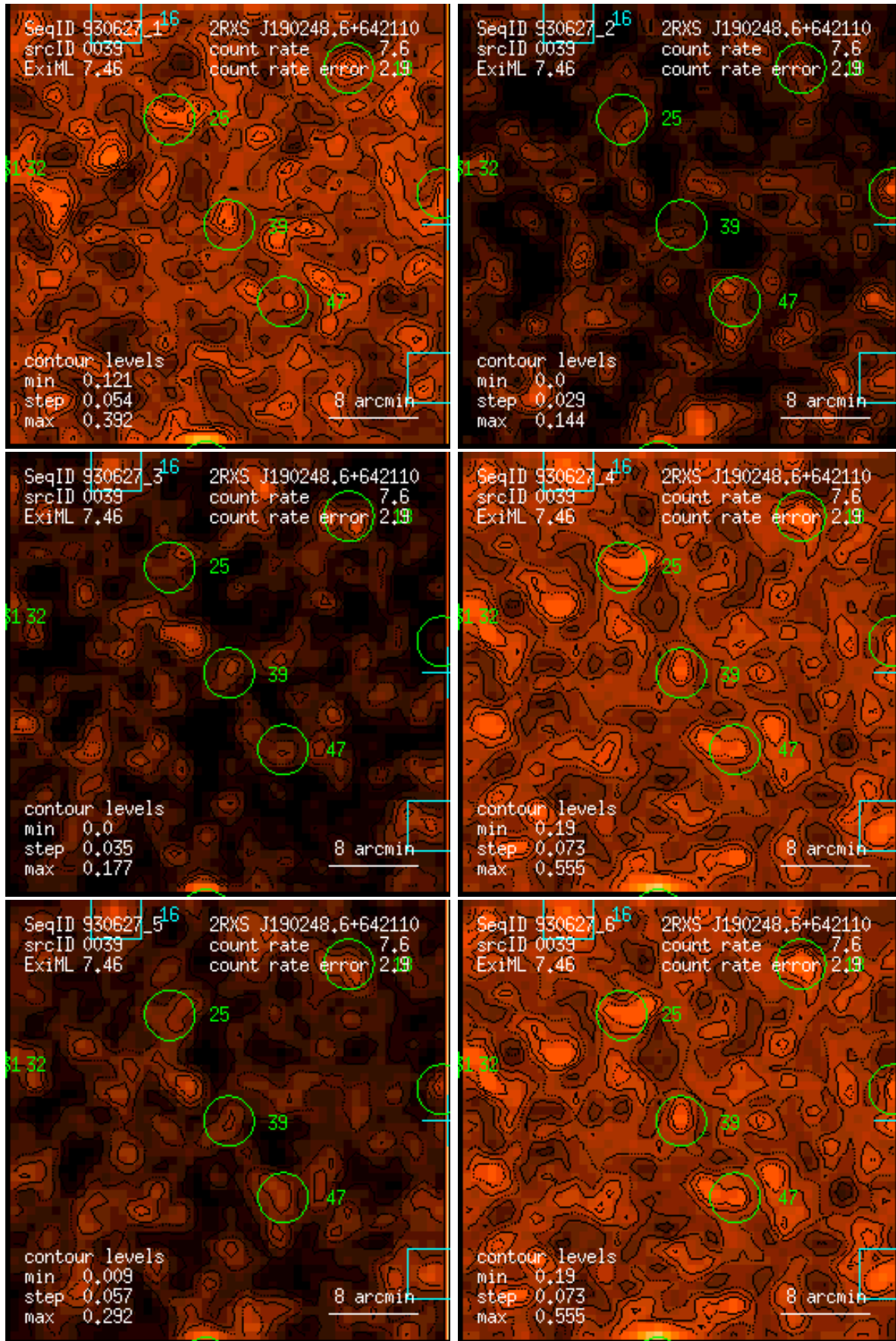
Figure 39: RASS 930627: detection 0039: band rate images, Gaussian filter: (1) PSPC channels 11 – 41, (2) 52 – 90, (3) 91 – 201, (4) 11 – 235, (5) 52 – 201, (6) 11 – 201. Broad band rates in counts/ks. Band rate contour levels in counts/ks/arcmin 2 .
