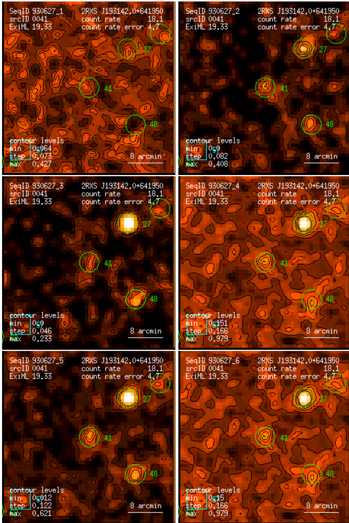
Figure 41: RASS 930627: detection 0041: band rate images, Gaussian filter: (1) PSPC channels 11 – 41, (2) 52 – 90, (3) 91 – 201, (4) 11 – 235, (5) 52 – 201, (6) 11 – 201. Broad band rates in counts/ks. Band rate contour levels in counts/ks/arcmin 2 .
