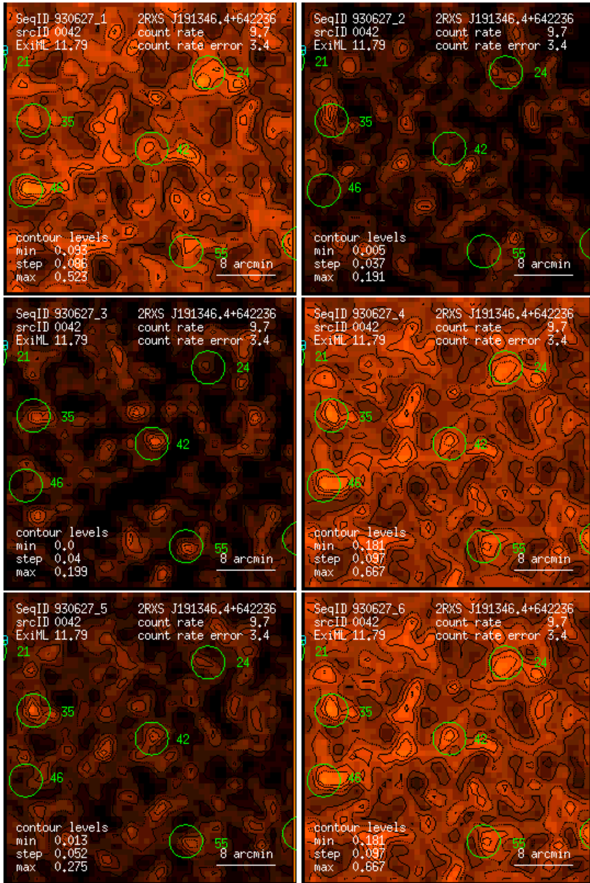
Figure 42: RASS 930627: detection 0042: band rate images, Gaussian filter: (1) PSPC channels 11 – 41, (2) 52 – 90, (3) 91 – 201, (4) 11 – 235, (5) 52 – 201, (6) 11 – 201. Broad band rates in counts/ks. Band rate contour levels in counts/ks/arcmin 2 .
