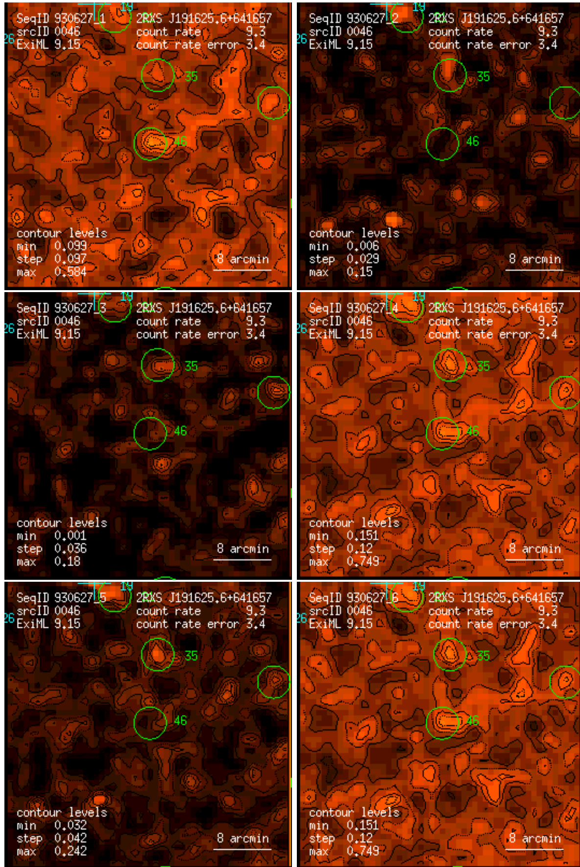
Figure 46: RASS 930627: detection 0046: band rate images, Gaussian filter: (1) PSPC channels 11 – 41, (2) 52 – 90, (3) 91 – 201, (4) 11 – 235, (5) 52 – 201, (6) 11 – 201. Broad band rates in counts/ks. Band rate contour levels in counts/ks/arcmin 2 .
