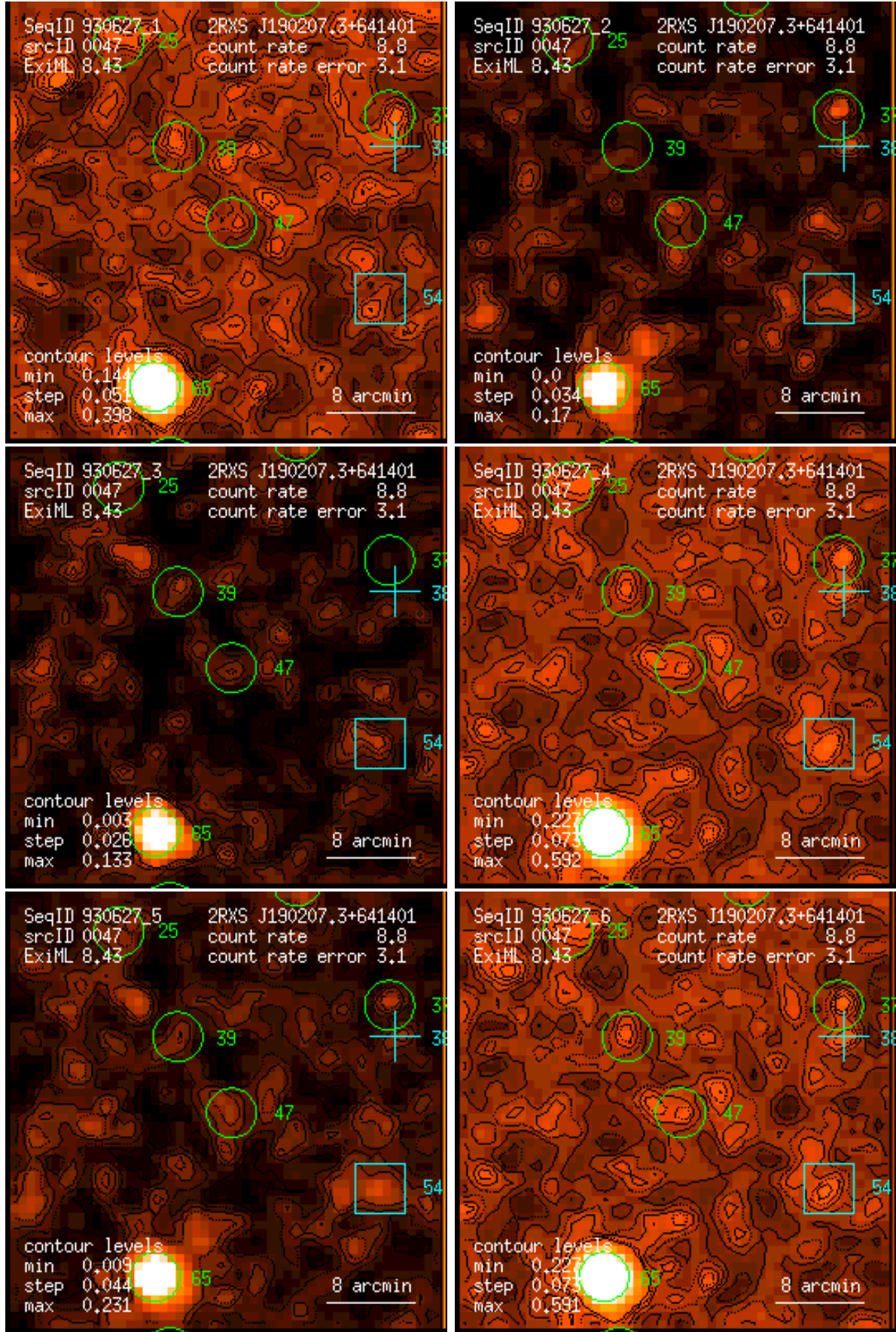
Figure 47: RASS 930627: detection 0047: band rate images, Gaussian filter: (1) PSPC channels 11 – 41, (2) 52 – 90, (3) 91 – 201, (4) 11 – 235, (5) 52 – 201, (6) 11 – 201. Broad band rates in counts/ks. Band rate contour levels in counts/ks/arcmin 2 .
