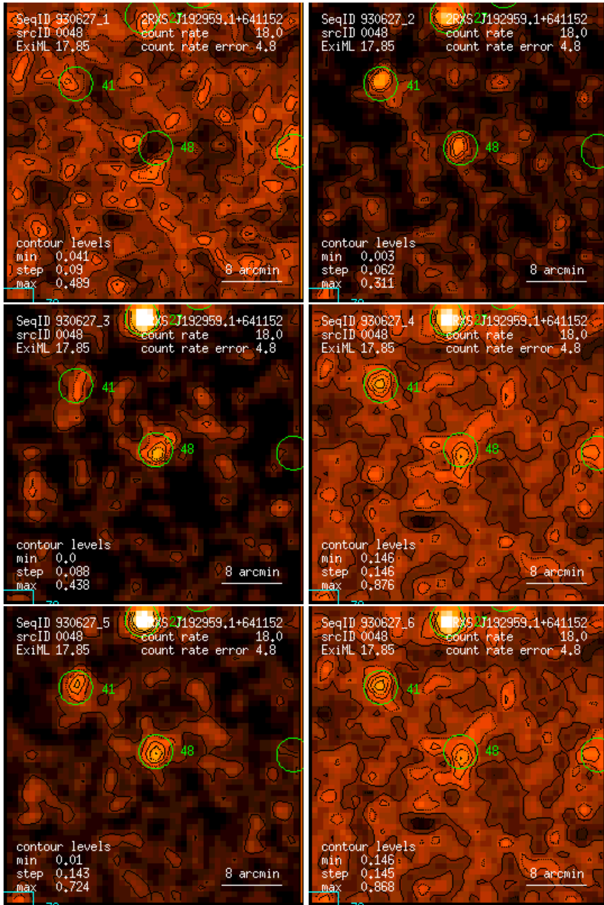
Figure 48: RASS 930627: detection 0048: band rate images, Gaussian filter: (1) PSPP channels 11 – 41, (2) 52 – 90, (3) 91 – 201, (4) 11 – 235, (5) 52 – 201, (6) 11 – 201. Broad band rates in counts/ks. Band rate contour levels in counts/ks/arcmin 2 .
