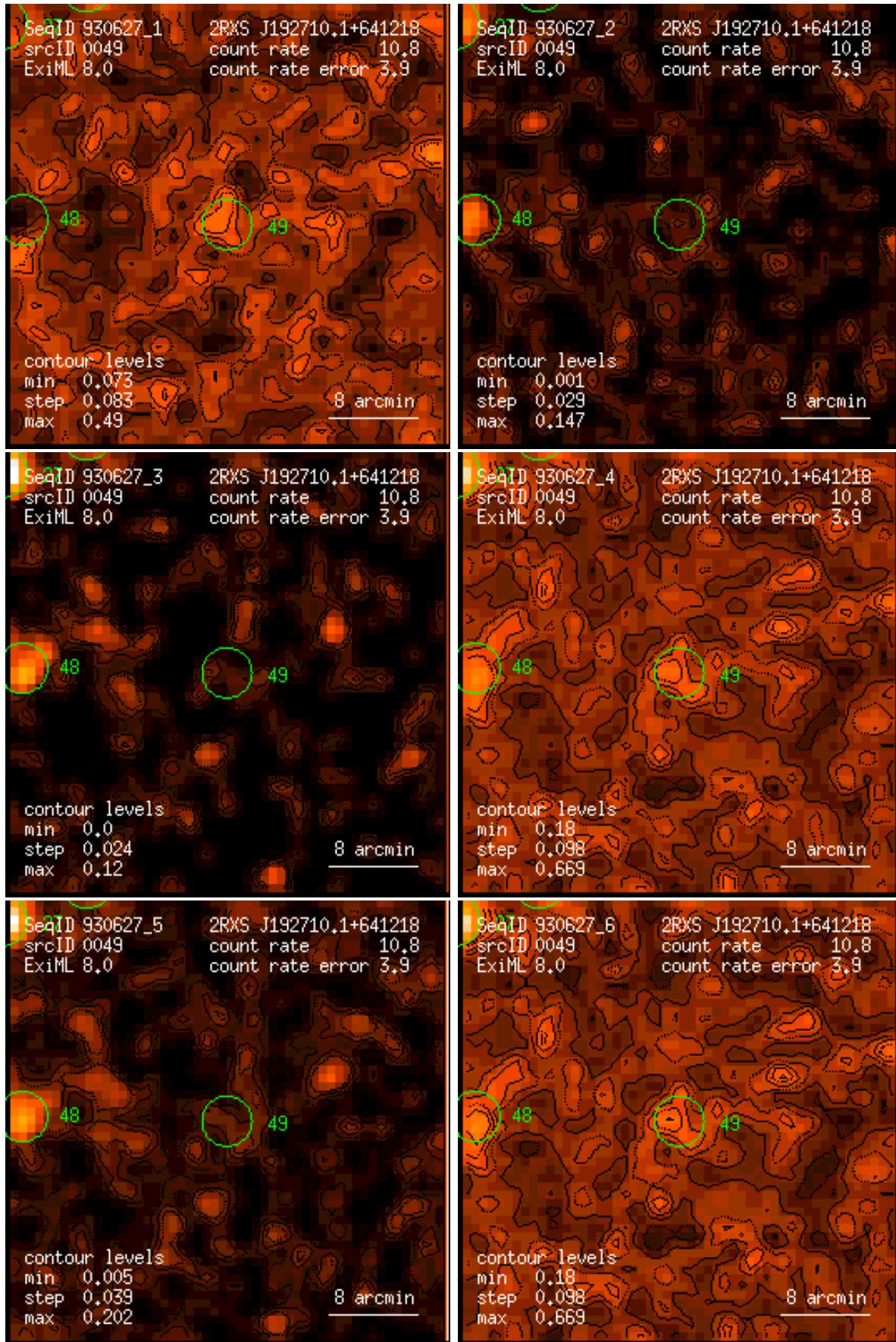
Figure 49: RASS 930627: detection 0049: band rate images, Gaussian filter: (1) PSPC channels 11 – 41, (2) 52 – 90, (3) 91 – 201, (4) 11 – 235, (5) 52 – 201, (6) 11 – 201. Broad band rates in counts/ks. Band rate contour levels in counts/ks/arcmin 2 .
