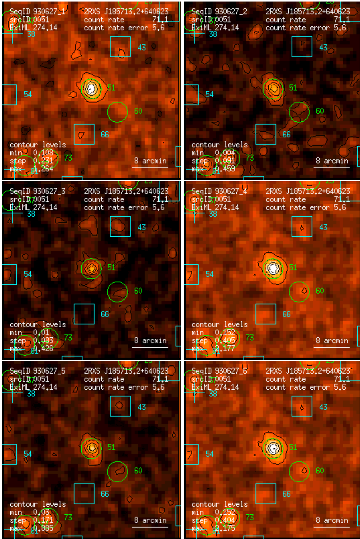
Figure 51: RASS 930627: detection 0051: band rate images, Gaussian filter: (1) PSPC channels 11 – 41, (2) 52 – 90, (3) 91 – 201, (4) 11 – 235, (5) 52 – 201, (6) 11 – 201. Broad band rates in counts/ks. Band rate contour levels in counts/ks/arcmin 2 .
