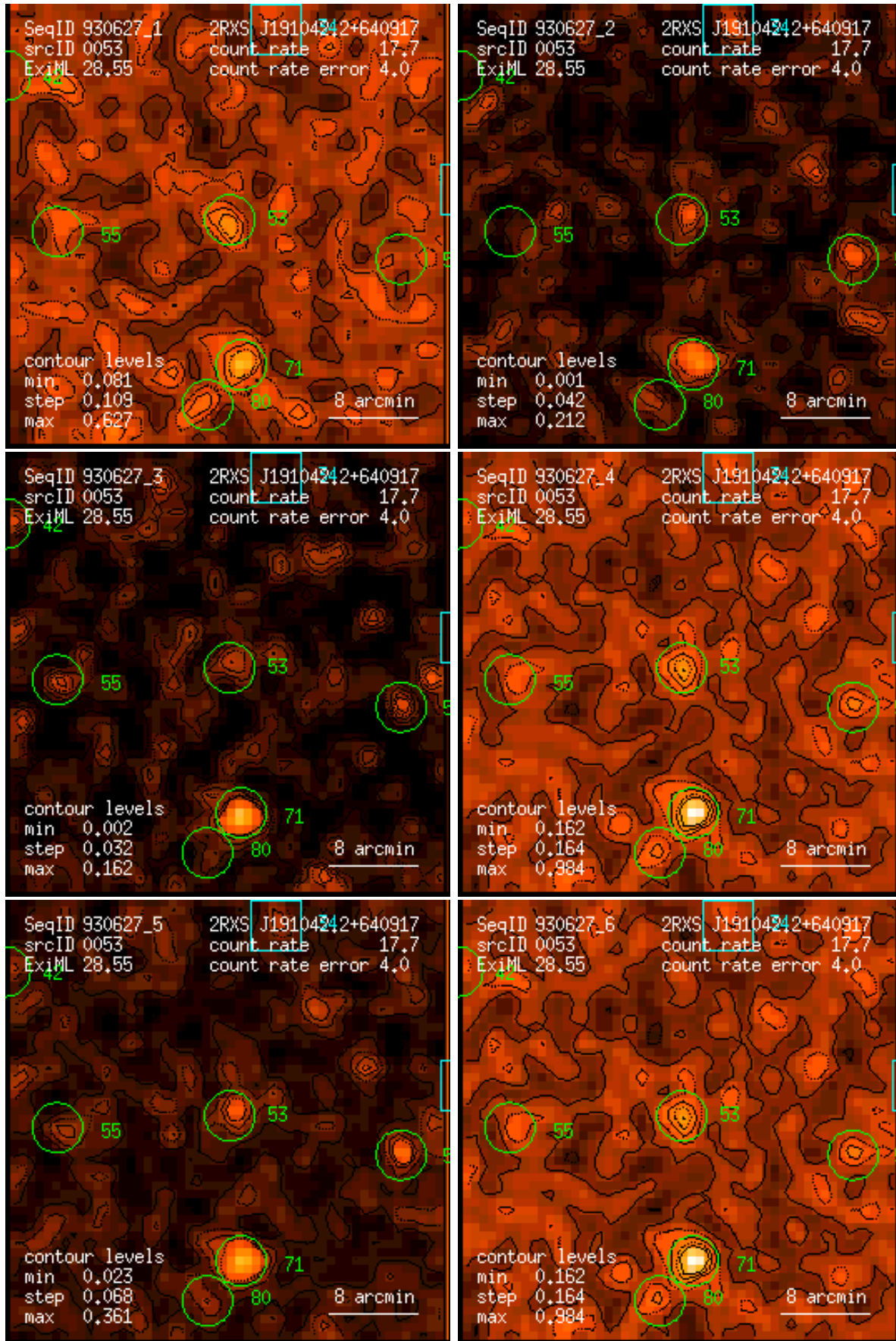
Figure 53: RASS 930627: detection 0053: band rate images, Gaussian filter: (1) PSPC channels 11 – 41, (2) 52 – 90, (3) 91 – 201, (4) 11 – 235, (5) 52 – 201, (6) 11 – 201. Broad band rates in counts/ks. Band rate contour levels in counts/ks/arcmin 2 .
