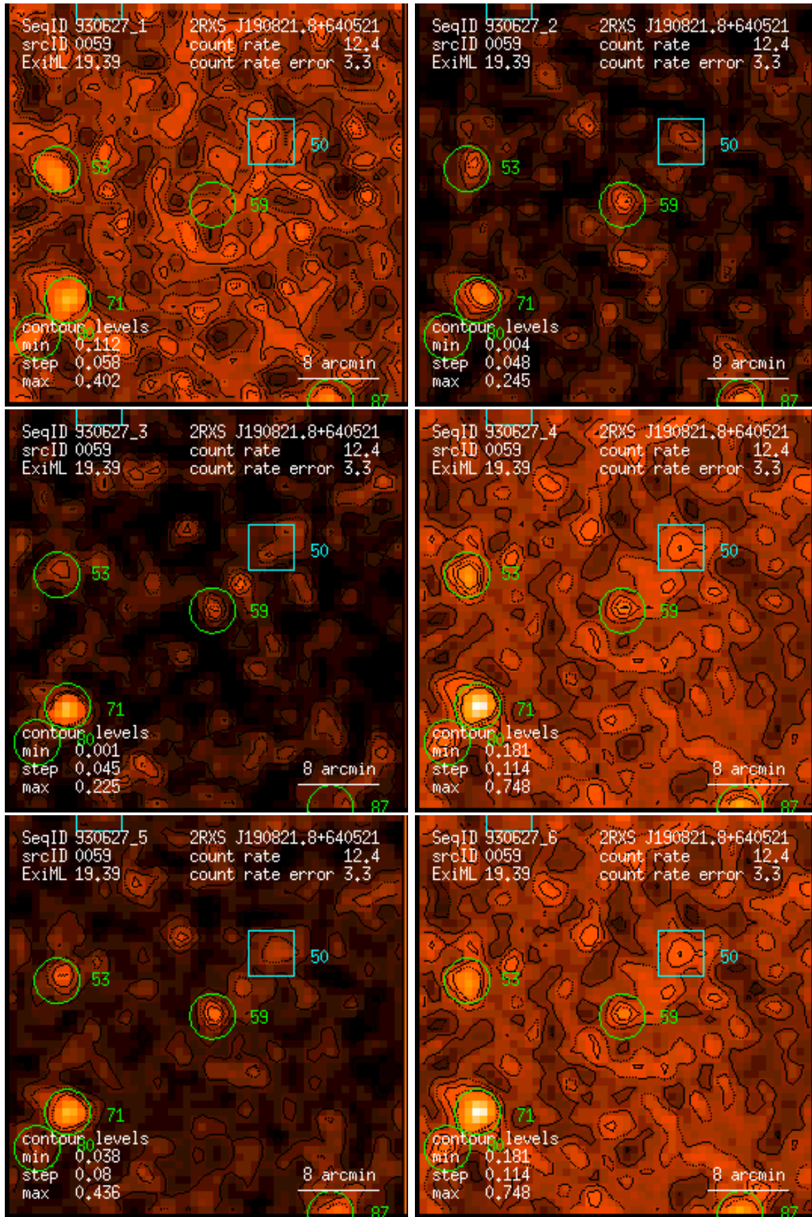
Figure 59: RASS 930627: detection 0059: band rate images, Gaussian filter: (1) PSPC channels 11 – 41, (2) 52 – 90, (3) 91 – 201, (4) 11 – 235, (5) 52 – 201, (6) 11 – 201. Broad band rates in counts/ks. Band rate contour levels in counts/ks/arcmin 2 .
