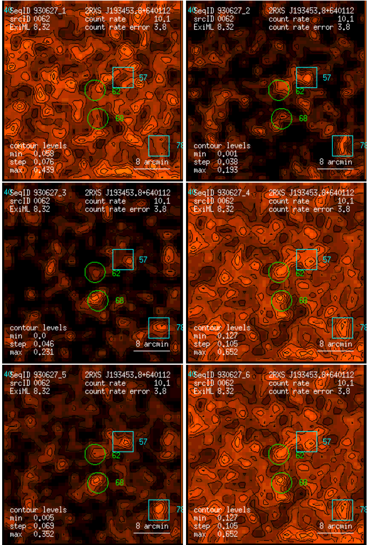
Figure 62: RASS 930627: detection 0062: band rate images, Gaussian filter: (1) PSPC channels 11 – 41, (2) 52 – 90, (3) 91 – 201, (4) 11 – 235, (5) 52 – 201, (6) 11 – 201. Broad band rates in counts/ks. Band rate contour levels in counts/ks/arcmin 2 .
