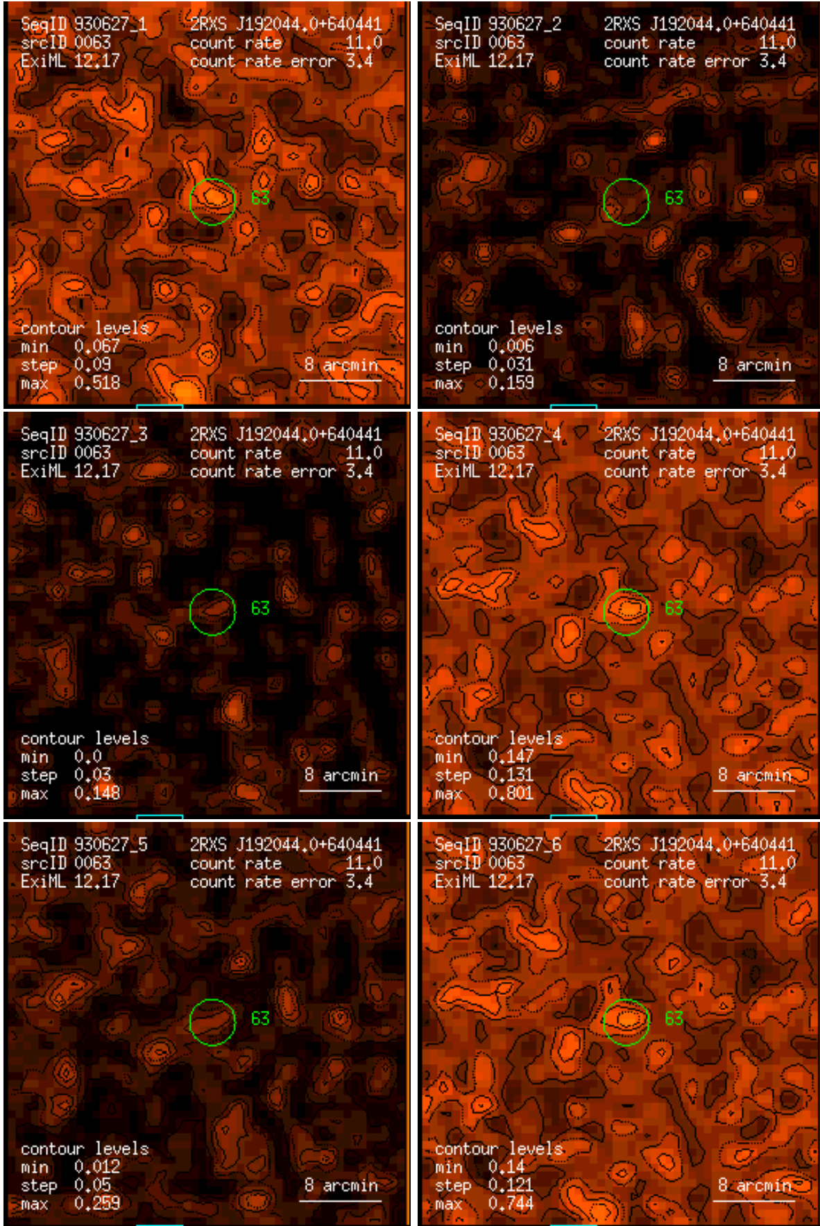
Figure 63: RASS 930627: detection 0063: band rate images, Gaussian filter: (1) PSPC channels 11 – 41, (2) 52 – 90, (3) 91 – 201, (4) 11 – 235, (5) 52 – 201, (6) 11 – 201. Broad band rates in counts/ks. Band rate contour levels in counts/ks/arcmin 2 .
