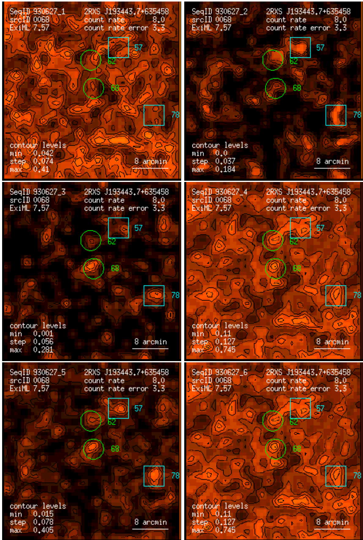
Figure 68: RASS 930627: detection 0068: band rate images, Gaussian filter: (1) PSPC channels 11 – 41, (2) 52 – 90, (3) 91 – 201, (4) 11 – 235, (5) 52 – 201, (6) 11 – 201. Broad band rates in counts/ks. Band rate contour levels in counts/ks/arcmin 2 .
