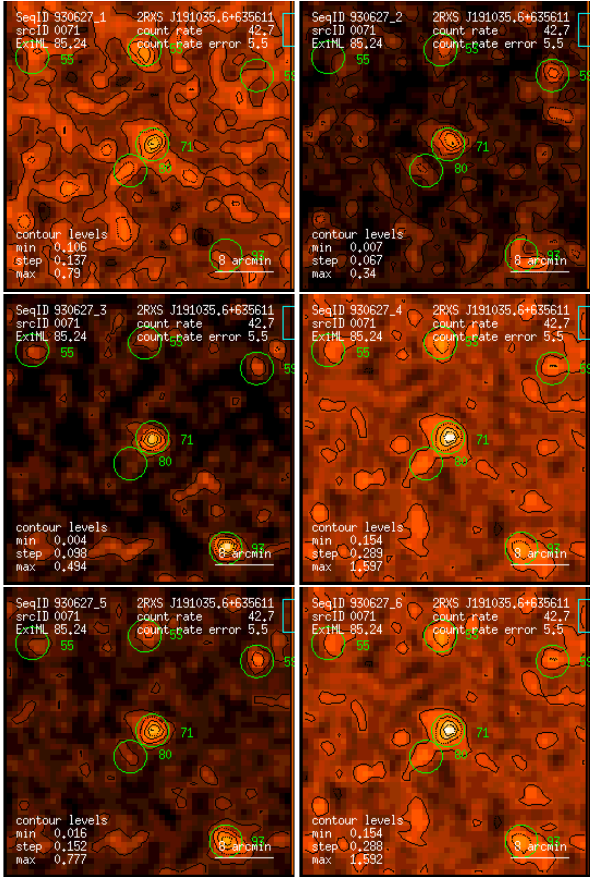
Figure 71: RASS 930627: detection 0071: band rate images, Gaussian filter: (1) PSPC channels 11 – 41, (2) 52 – 90, (3) 91 – 201, (4) 11 – 235, (5) 52 – 201, (6) 11 – 201. Broad band rates in counts/ks. Band rate contour levels in counts/ks/arcmin 2 .
