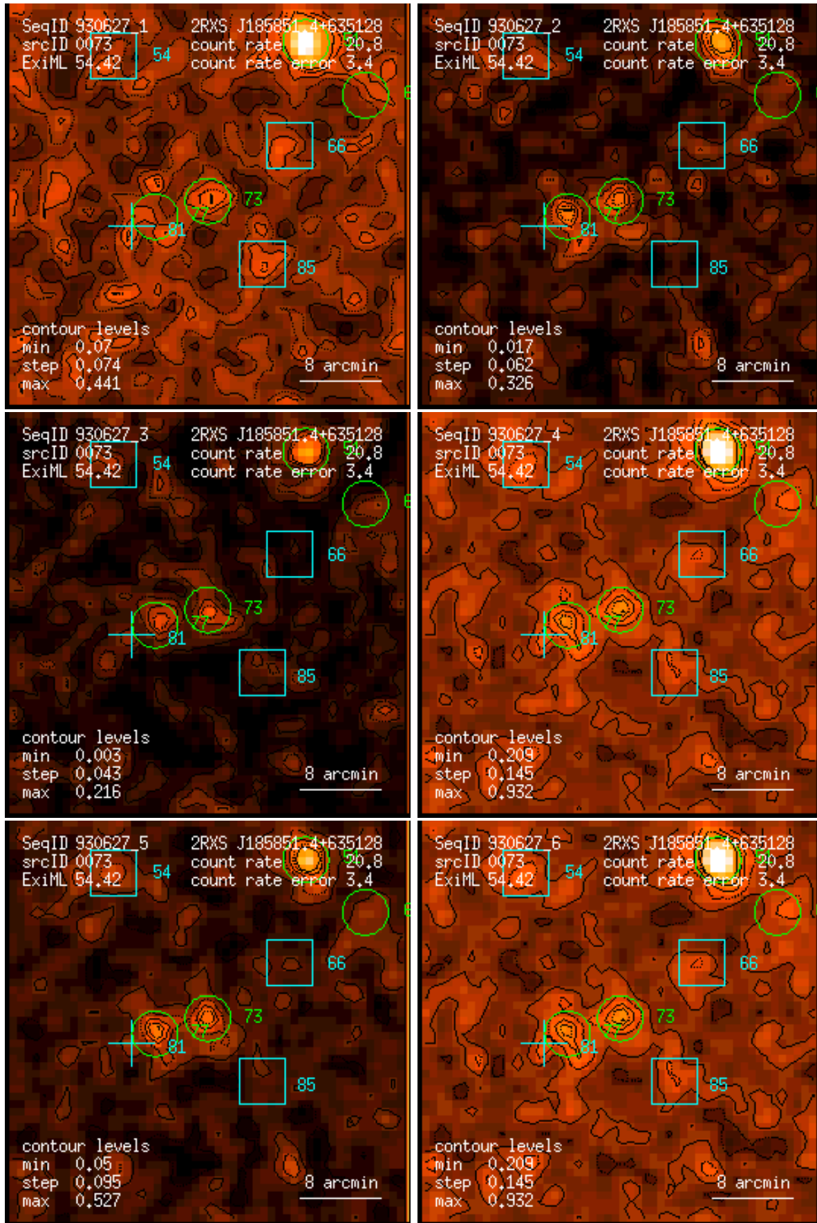
Figure 73: RASS 930627: detection 0073: band rate images, Gaussian filter: (1) PSPC channels 11 – 41, (2) 52 – 90, (3) 91 – 201, (4) 11 – 235, (5) 52 – 201, (6) 11 – 201. Broad band rates in counts/ks. Band rate contour levels in counts/ks/arcmin 2 .
