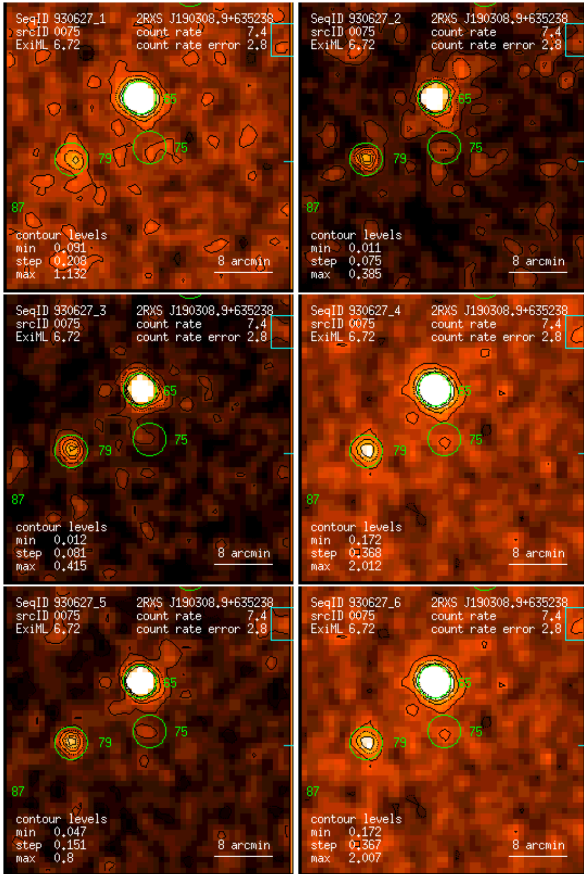
Figure 75: RASS 930627: detection 0075: band rate images, Gaussian filter: (1) PSPC channels 11 – 41, (2) 52 – 90, (3) 91 – 201, (4) 11 – 235, (5) 52 – 201, (6) 11 – 201. Broad band rates in counts/ks. Band rate contour levels in counts/ks/arcmin 2 .
