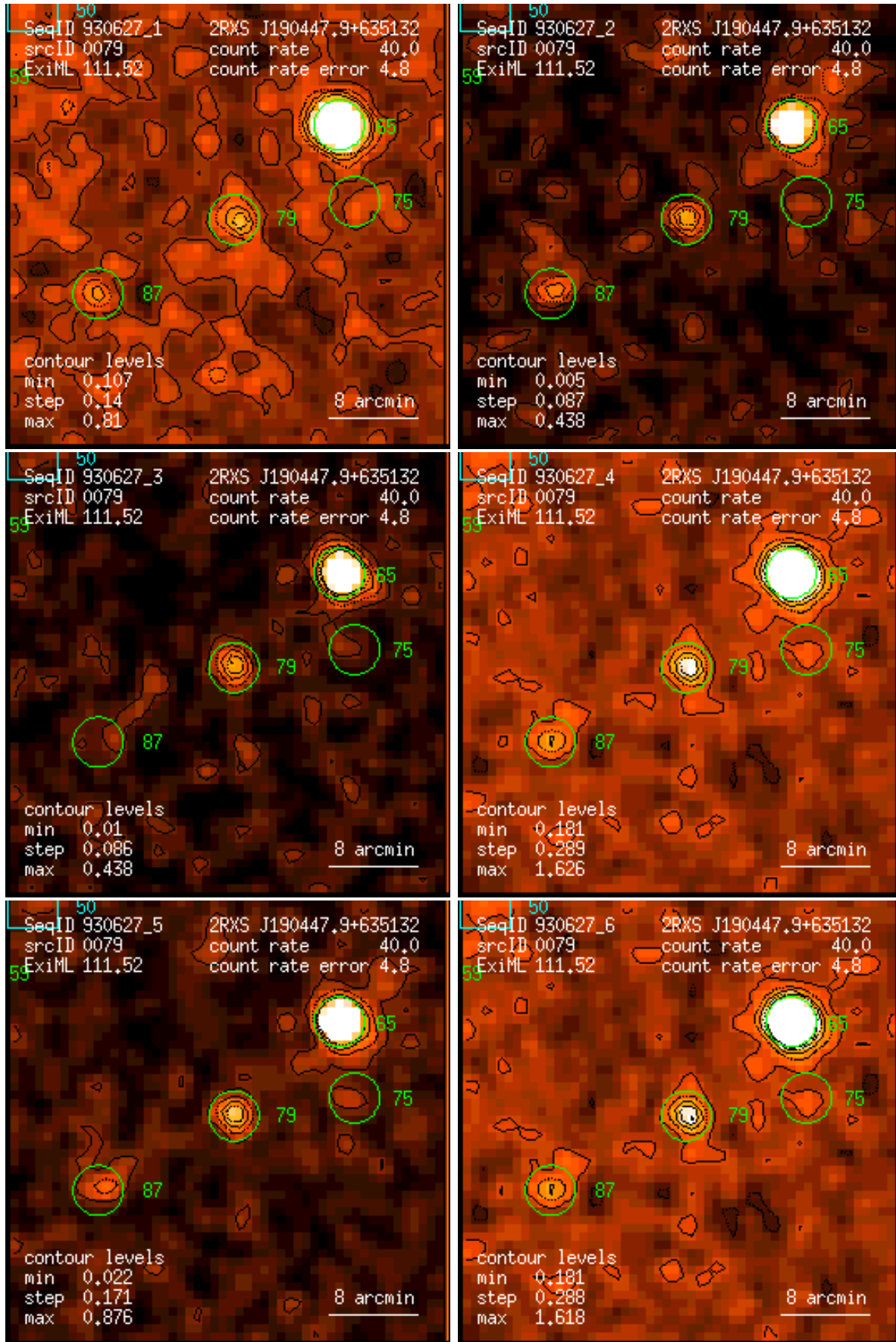
Figure 79: RASS 930627: detection 0079: band rate images, Gaussian filter: (1) PSPC channels 11 – 41, (2) 52 – 90, (3) 91 – 201, (4) 11 – 235, (5) 52 – 201, (6) 11 – 201. Broad band rates in counts/ks. Band rate contour levels in counts/ks/arcmin 2 .
