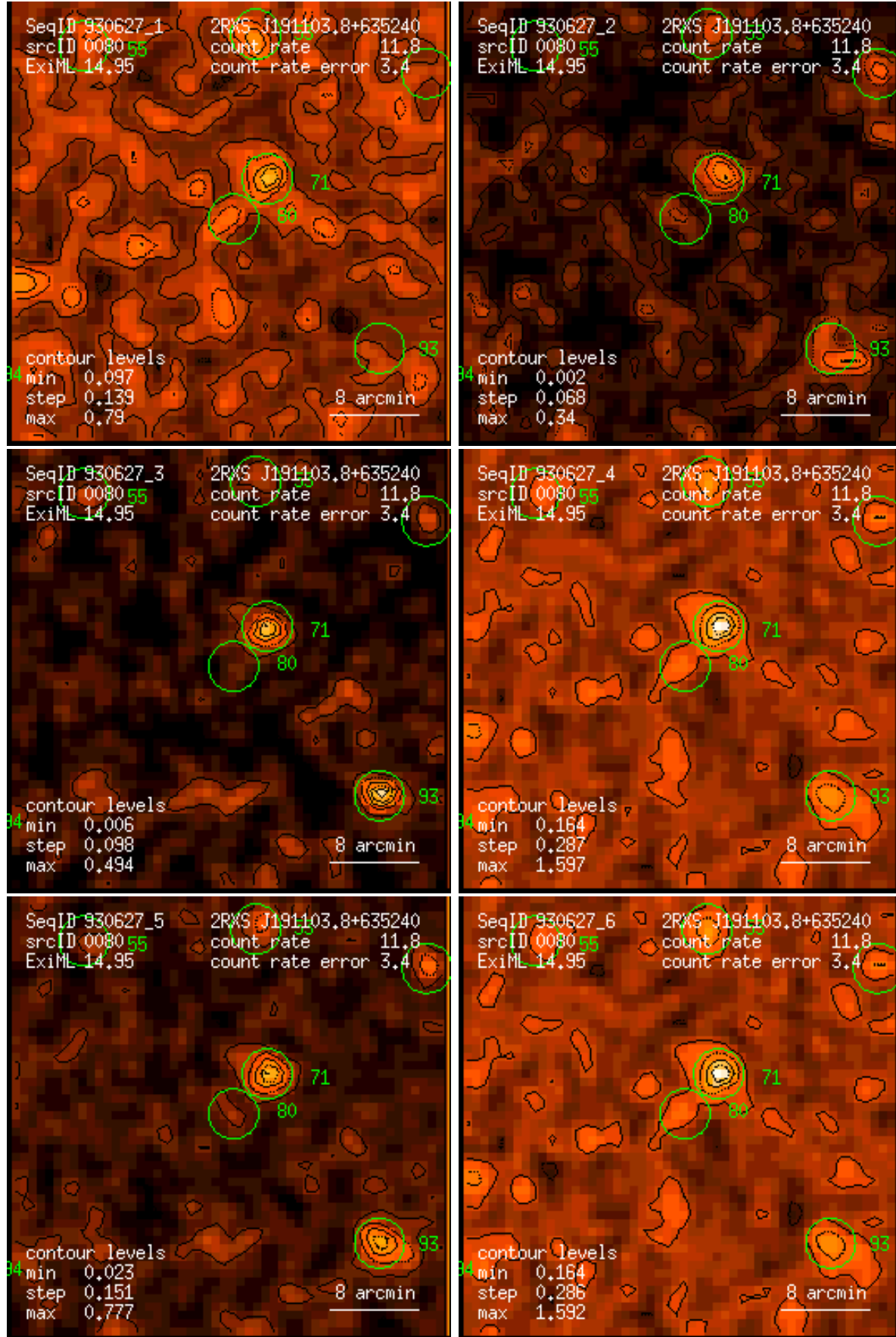
Figure 80: RASS 930627: detection 0080: band rate images, Gaussian filter: (1) PSPC channels 11 – 41, (2) 52 – 90, (3) 91 – 201, (4) 11 – 235, (5) 52 – 201, (6) 11 – 201. Broad band rates in counts/ks. Band rate contour levels in counts/ks/arcmin 2 .
