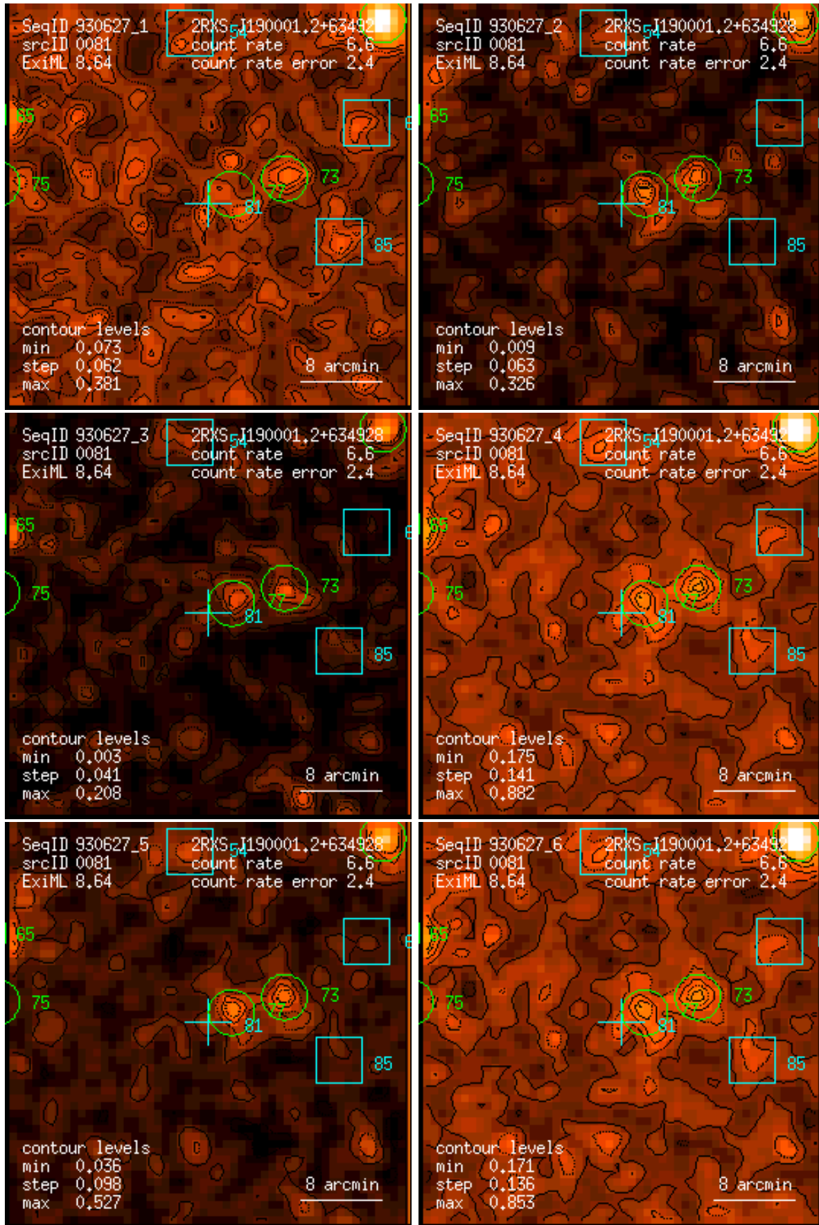
Figure 81: RASS 930627: detection 0081: band rate images, Gaussian filter: (1) PSPC channels 11 – 41, (2) 52 – 90, (3) 91 – 201, (4) 11 – 235, (5) 52 – 201, (6) 11 – 201. Broad band rates in counts/ks. Band rate contour levels in counts/ks/arcmin 2 .
