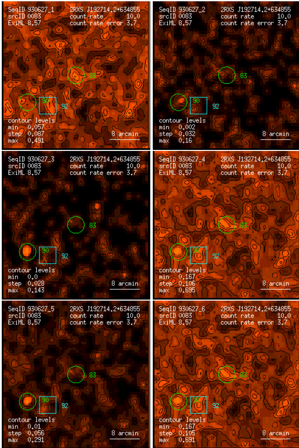
Figure 83: RASS 930627: detection 0083: band rate images, Gaussian filter: (1) PSPC channels 11 – 41, (2) 52 – 90, (3) 91 – 201, (4) 11 – 235, (5) 52 – 201, (6) 11 – 201. Broad band rates in counts/ks. Band rate contour levels in counts/ks/arcmin 2 .
