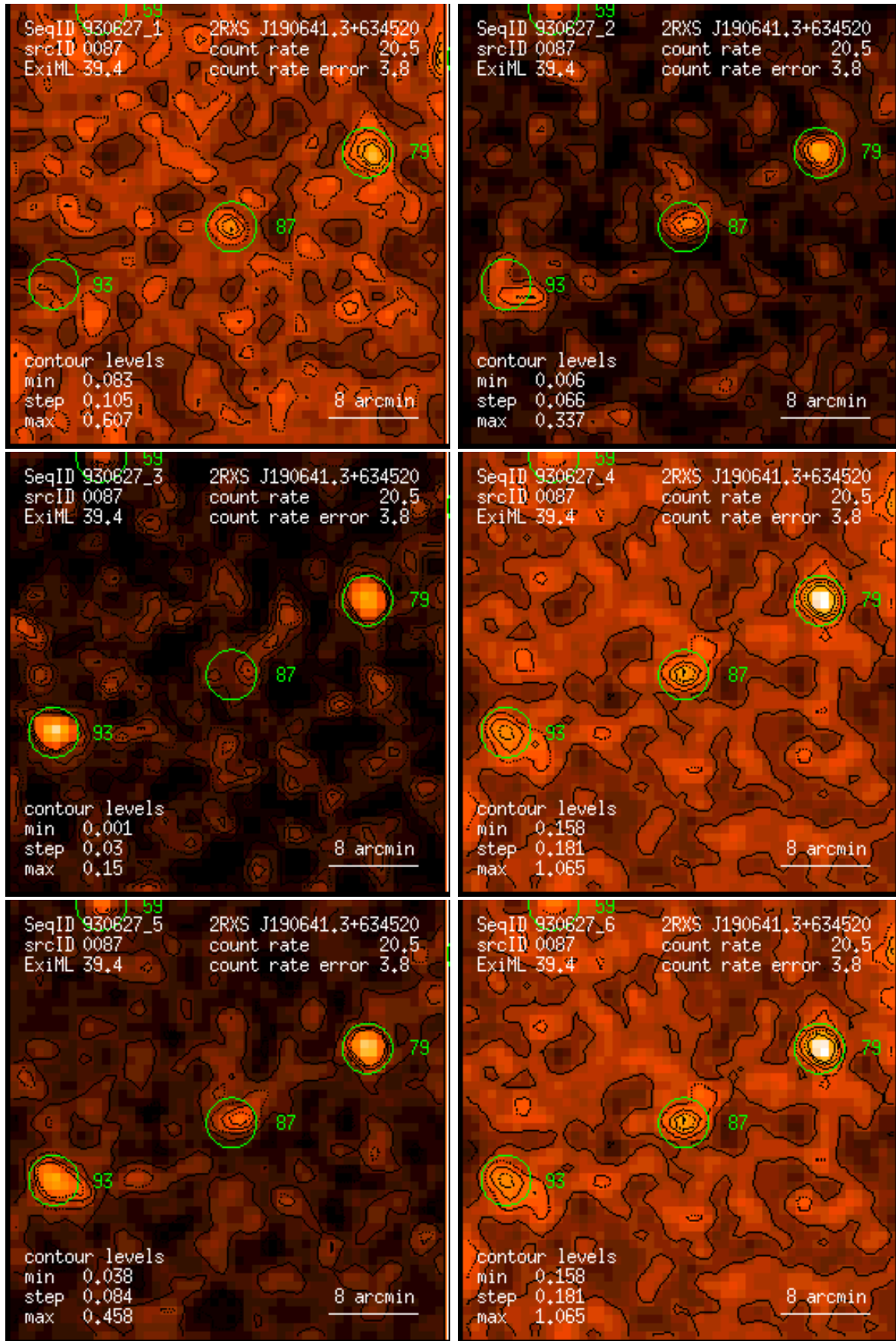
Figure 87: RASS 930627: detection 0087: band rate images, Gaussian filter: (1) PSPC channels 11 – 41, (2) 52 – 90, (3) 91 – 201, (4) 11 – 235, (5) 52 – 201, (6) 11 – 201. Broad band rates in counts/ks. Band rate contour levels in counts/ks/arcmin 2 .
