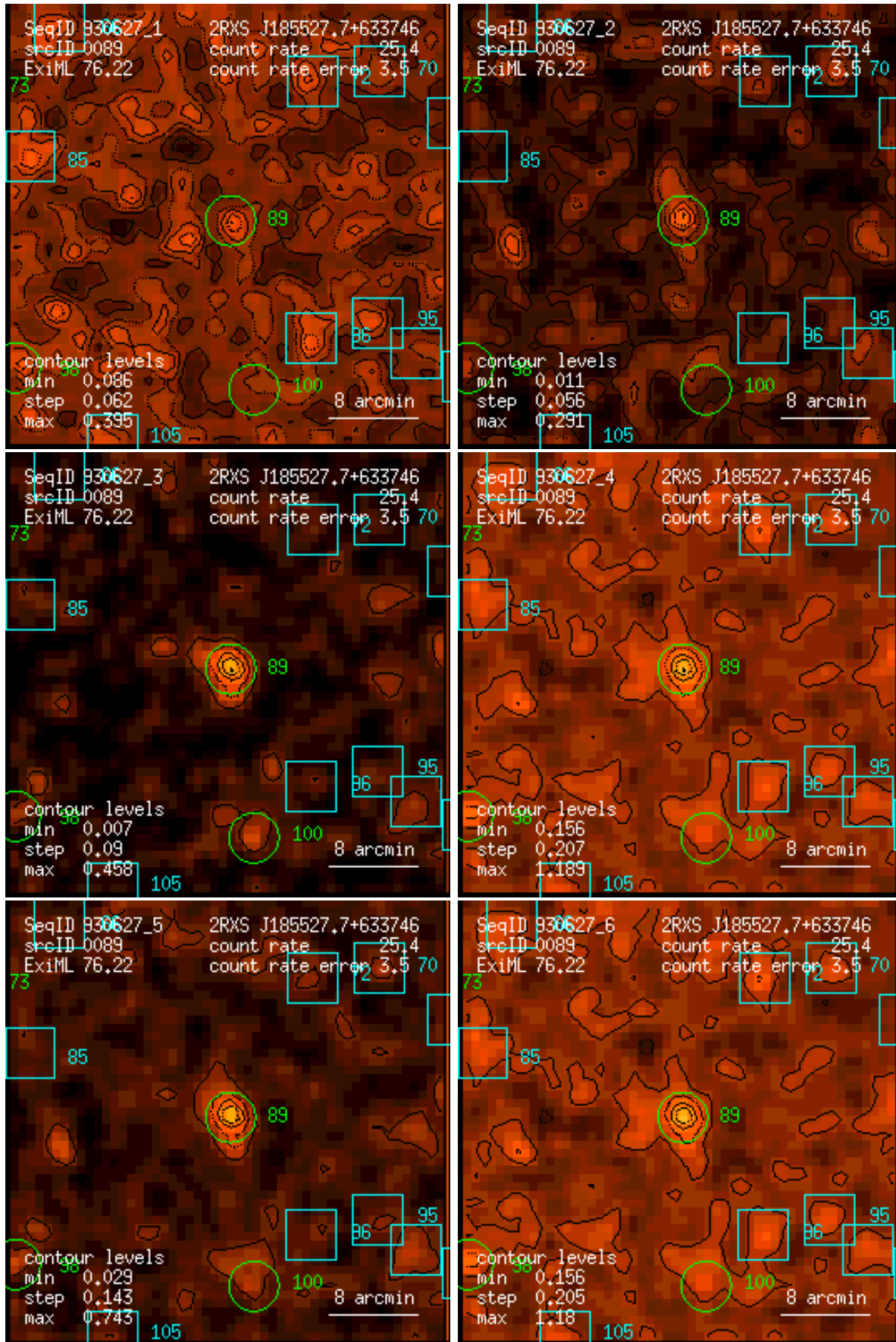
Figure 89: RASS 930627: detection 0089: band rate images, Gaussian filter: (1) PSPC channels 11 – 41, (2) 52 – 90, (3) 91 – 201, (4) 11 – 235, (5) 52 – 201, (6) 11 – 201. Broad band rates in counts/ks. Band rate contour levels in counts/ks/arcmin 2 .
