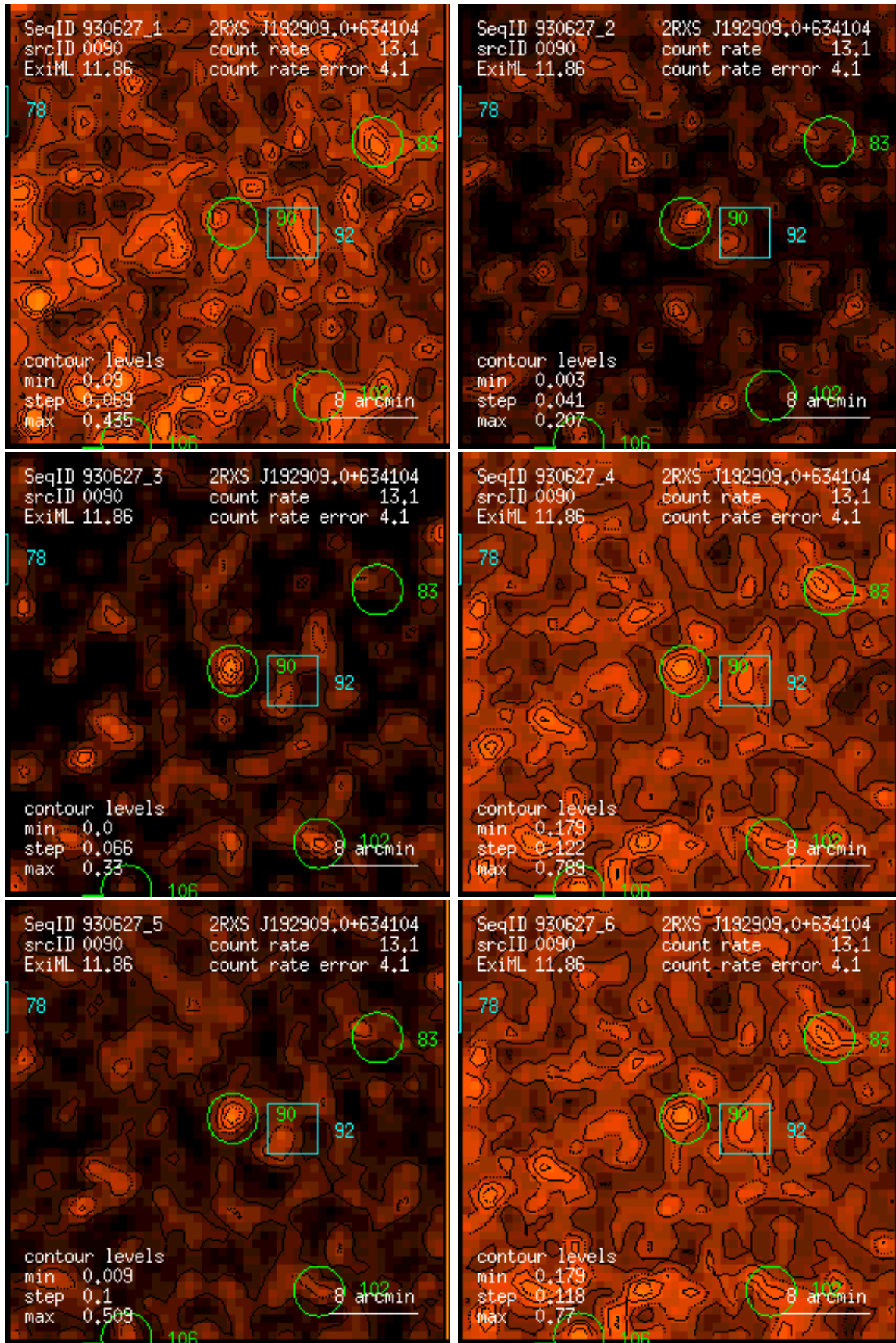
Figure 90: RASS 930627: detection 0090: band rate images, Gaussian filter: (1) PSPC channels 11 – 41, (2) 52 – 90, (3) 91 – 201, (4) 11 – 235, (5) 52 – 201, (6) 11 – 201. Broad band rates in counts/ks. Band rate contour levels in counts/ks/arcmin 2 .
