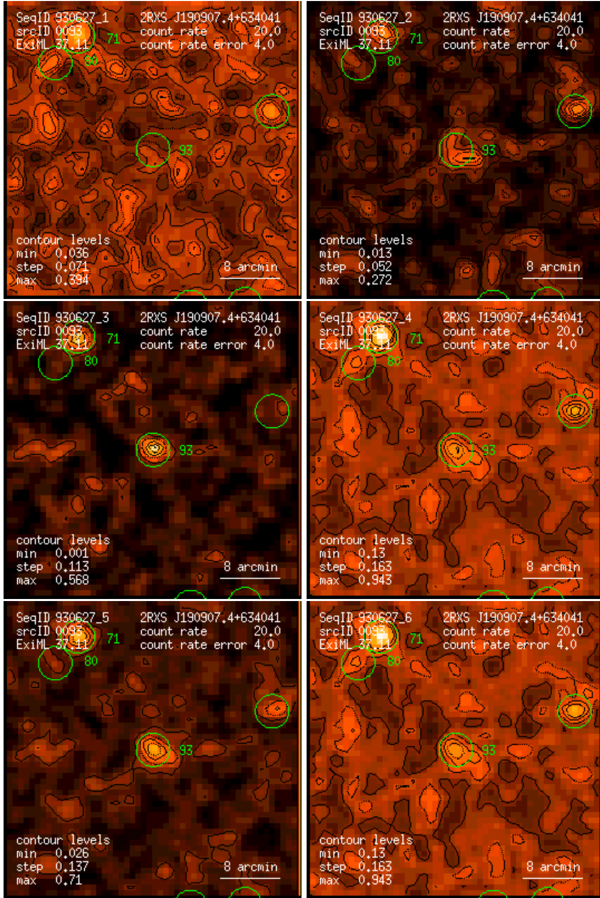
Figure 93: RASS 930627: detection 0093: band rate images, Gaussian filter: (1) PSPC channels 11 – 41, (2) 52 – 90, (3) 91 – 201, (4) 11 – 235, (5) 52 – 201, (6) 11 – 201. Broad band rates in counts/ks. Band rate contour levels in counts/ks/arcmin 2 .
