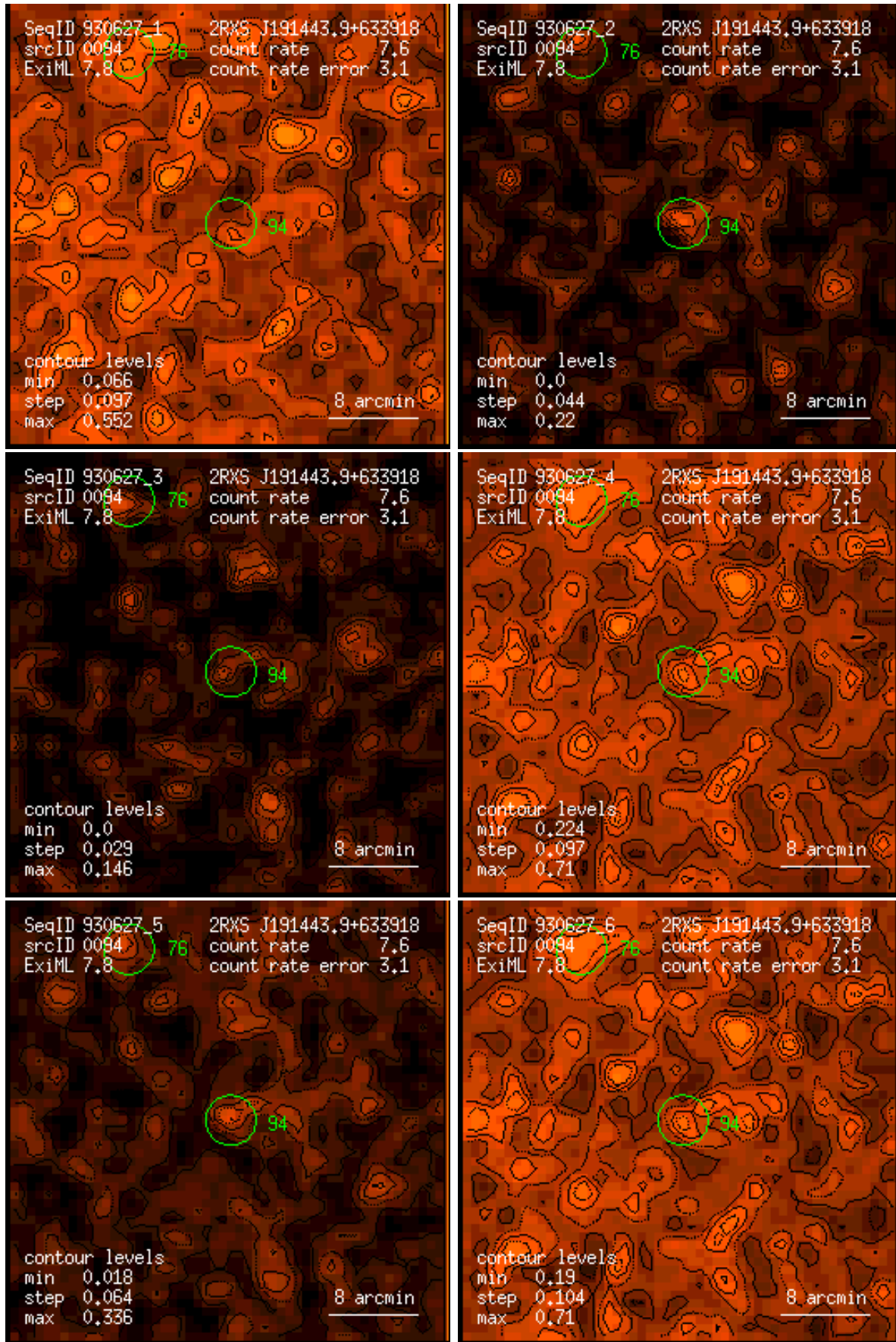
Figure 94: RASS 930627: detection 0094: band rate images, Gaussian filter: (1) PSPC channels 11 – 41, (2) 52 – 90, (3) 91 – 201, (4) 11 – 235, (5) 52 – 201, (6) 11 – 201. Broad band rates in counts/ks. Band rate contour levels in counts/ks/arcmin 2 .
