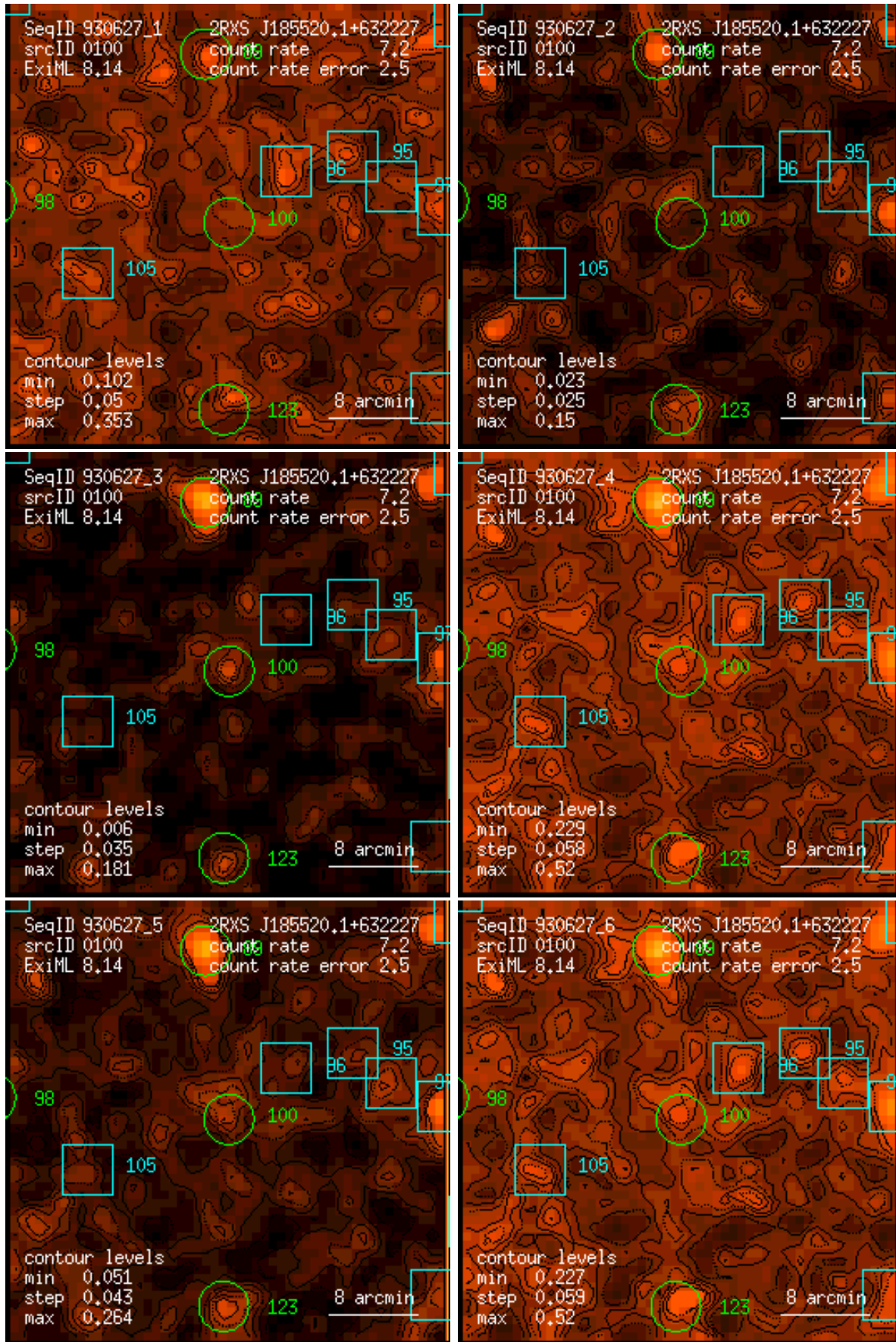
Figure 100: RASS 930627: detection 0100: band rate images, Gaussian filter: (1) PSPC channels 11 – 41, (2) 52 – 90, (3) 91 – 201, (4) 11 – 235, (5) 52 – 201, (6) 11 – 201. Broad band rates in counts/ks. Band rate contour levels in counts/ks/arcmin 2 .
