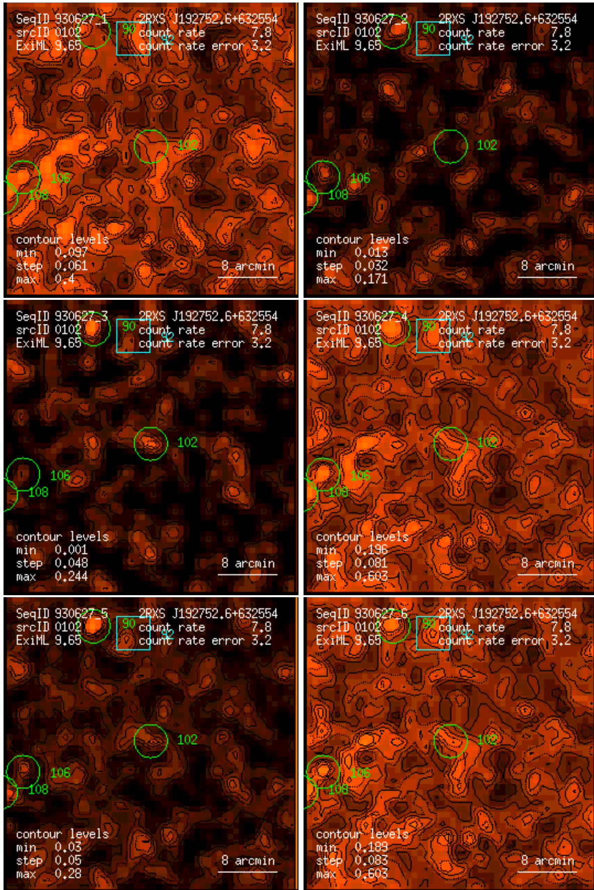
Figure 102: RASS 930627: detection 0102: band rate images, Gaussian filter: (1) PSPC channels 11 – 41, (2) 52 – 90, (3) 91 – 201, (4) 11 – 235, (5) 52 – 201, (6) 11 – 201. Broad band rates in counts/ks. Band rate contour levels in counts/ks/arcmin 2 .
