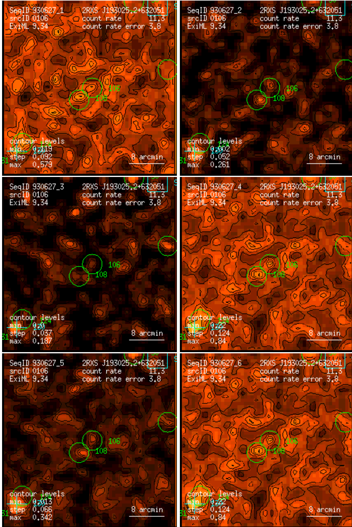
Figure 106: RASS 930627: detection 0106: band rate images, Gaussian filter: (1) PSPC channels 11 – 41, (2) 52 – 90, (3) 91 – 201, (4) 11 – 235, (5) 52 – 201, (6) 11 – 201. Broad band rates in counts/ks. Band rate contour levels in counts/ks/arcmin 2 .
