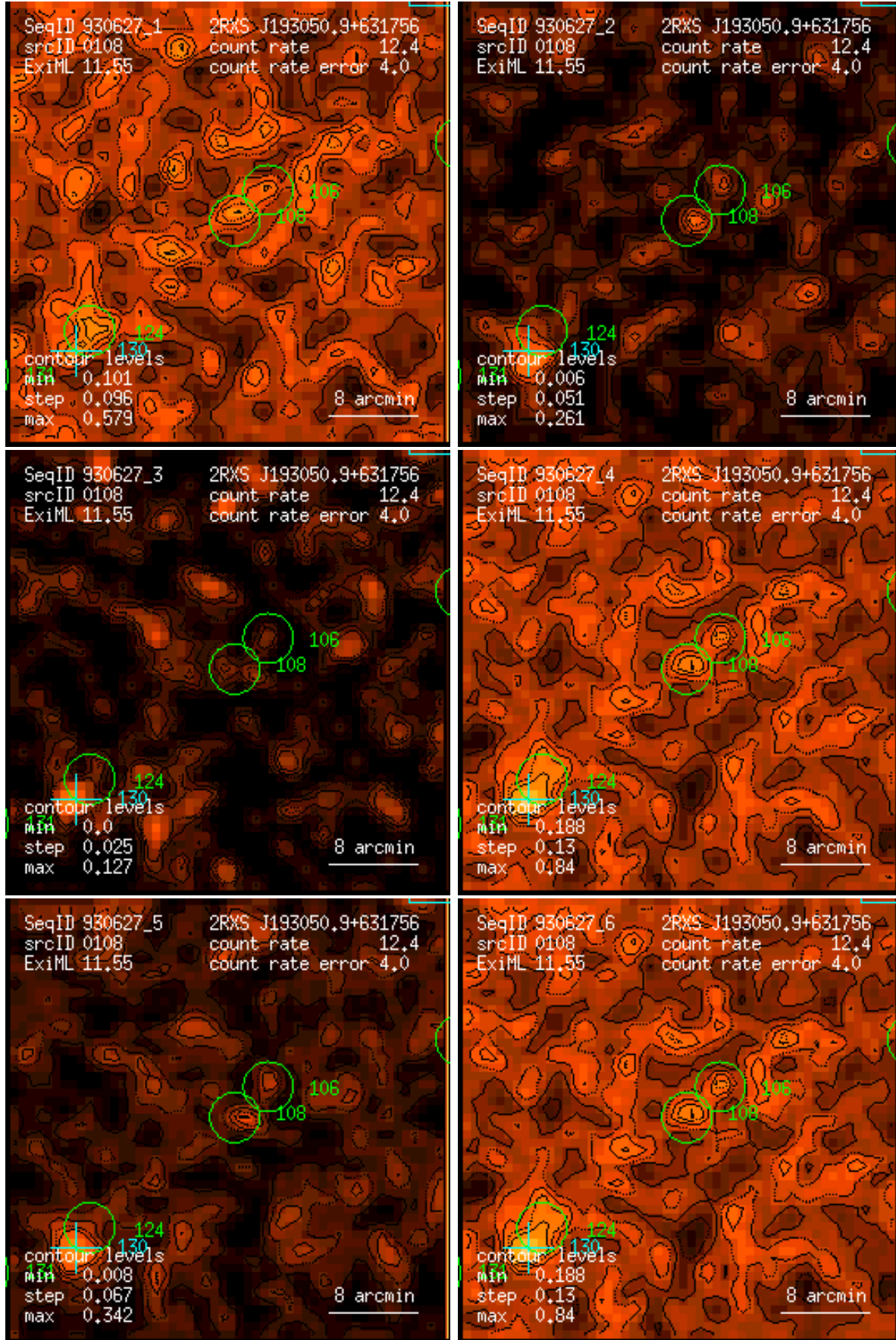
Figure 108: RASS 930627: detection 0108: band rate images, Gaussian filter: (1) PSPC channels 11 – 41, (2) 52 – 90, (3) 91 – 201, (4) 11 – 235, (5) 52 – 201, (6) 11 – 201. Broad band rates in counts/ks. Band rate contour levels in counts/ks/arcmin 2 .
