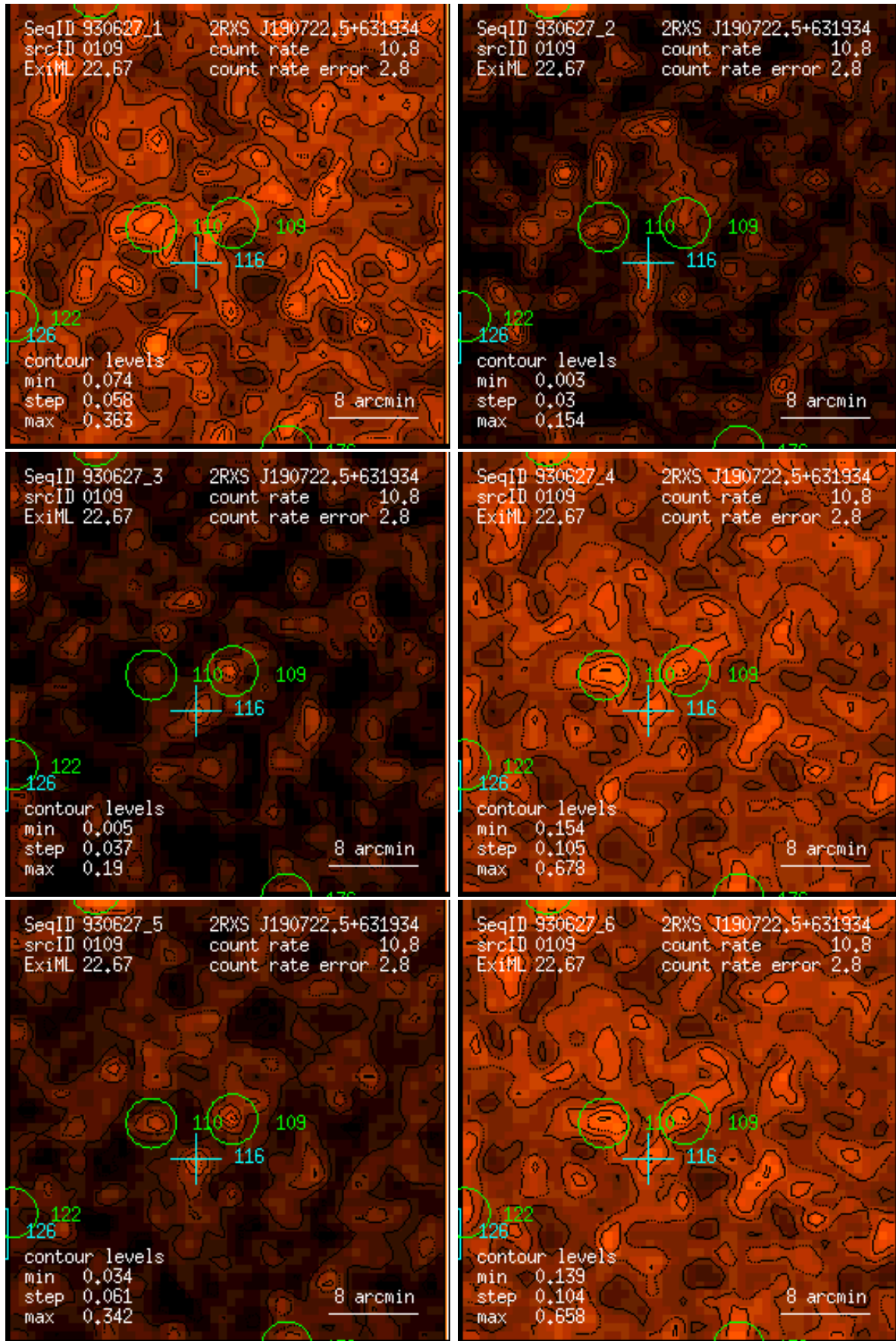
Figure 109: RASS 930627: detection 0109: band rate images, Gaussian filter: (1) PSPC channels 11 – 41, (2) 52 – 90, (3) 91 – 201, (4) 11 – 235, (5) 52 – 201, (6) 11 – 201. Broad band rates in counts/ks. Band rate contour levels in counts/ks/arcmin 2 .
