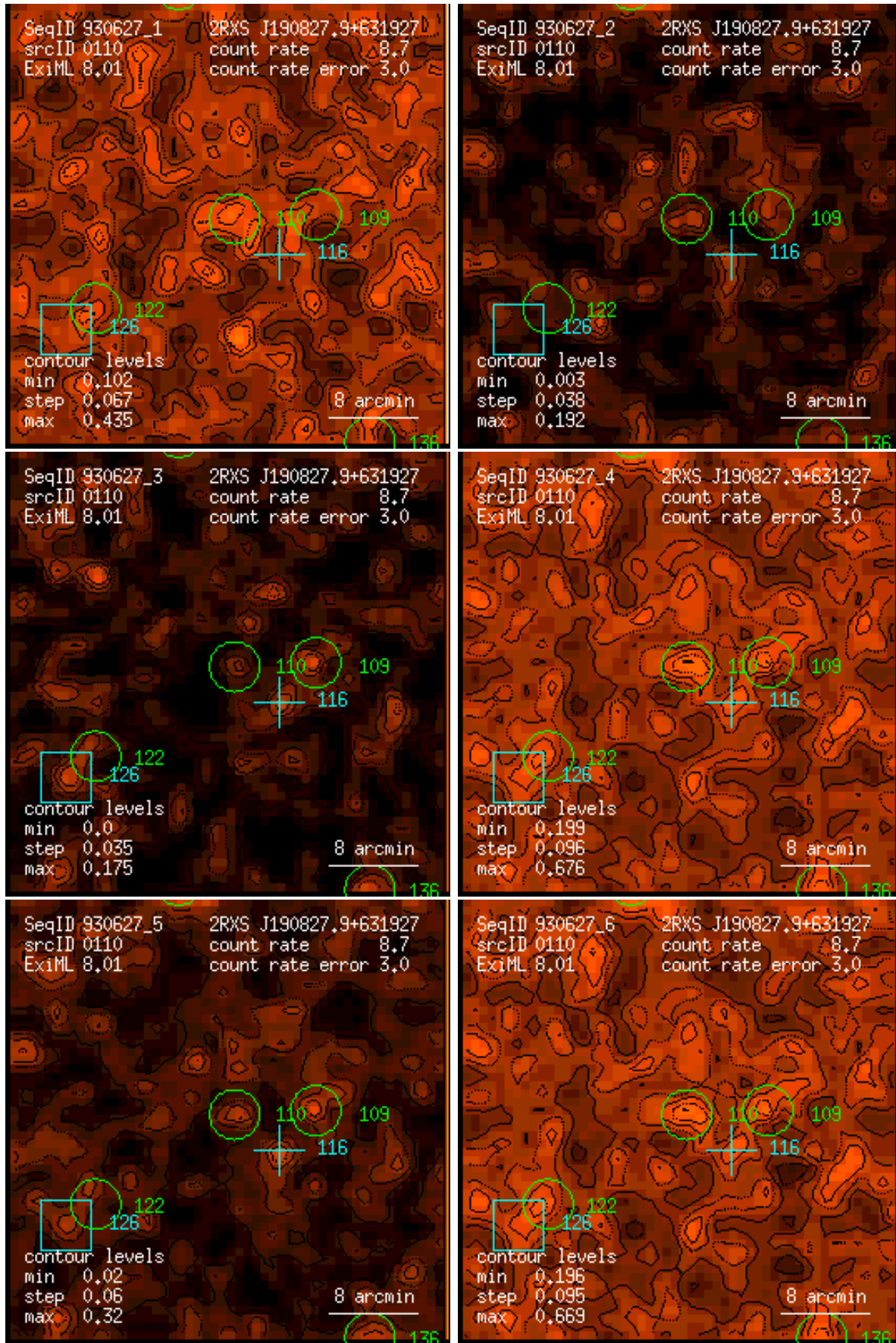
Figure 110: RASS 930627: detection 0110: band rate images, Gaussian filter: (1) PSPC channels 11 – 41, (2) 52 – 90, (3) 91 – 201, (4) 11 – 235, (5) 52 – 201, (6) 11 – 201. Broad band rates in counts/ks. Band rate contour levels in counts/ks/arcmin 2 .
