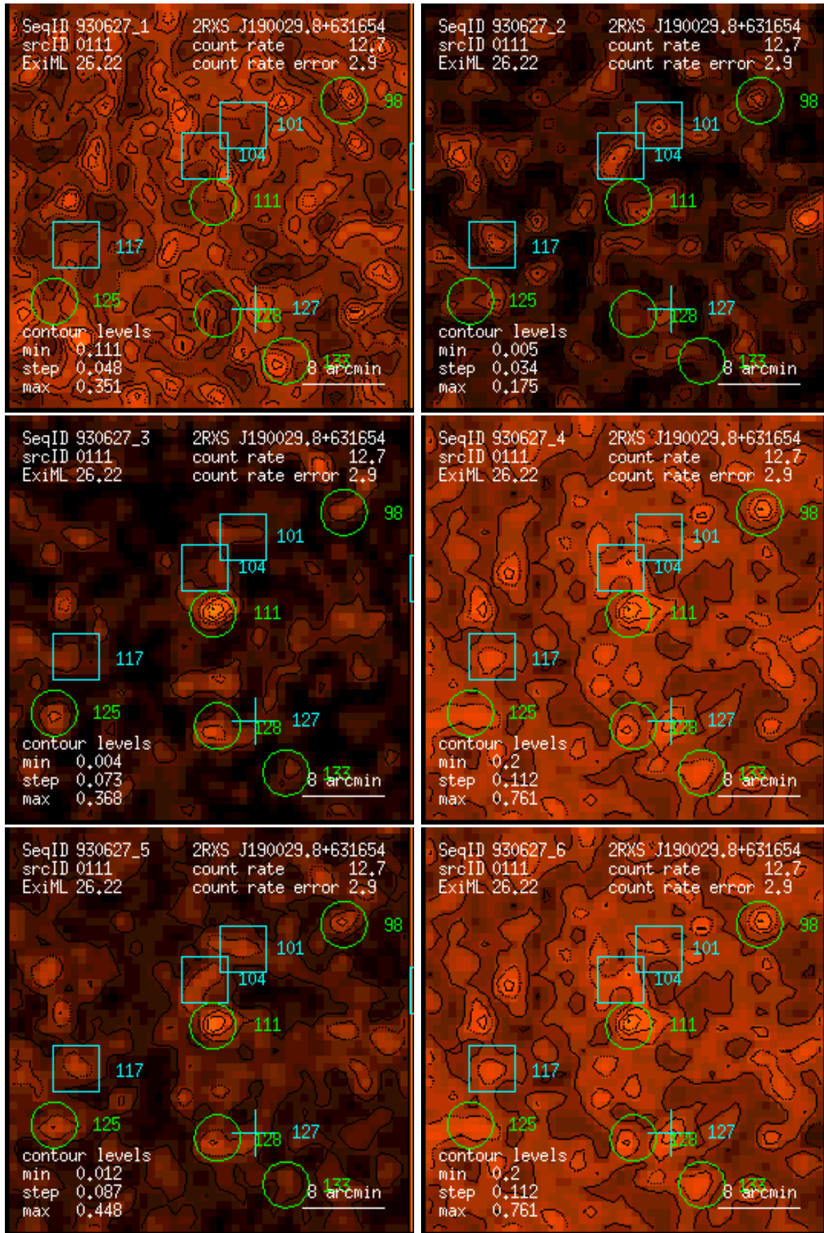
Figure 111: RASS 930627: detection 0111: band rate images, Gaussian filter: (1) PSPC channels 11 – 41, (2) 52 – 90, (3) 91 – 201, (4) 11 – 235, (5) 52 – 201, (6) 11 – 201. Broad band rates in counts/ks. Band rate contour levels in counts/ks/arcmin 2 .
