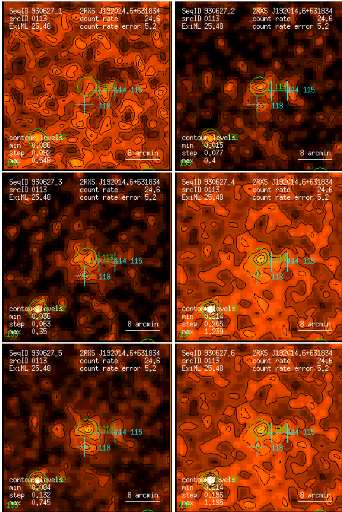
Figure 113: RASS 930627: detection 0113: band rate images, Gaussian filter: (1) PSPC channels 11 – 41, (2) 52 – 90, (3) 91 – 201, (4) 11 – 235, (5) 52 – 201, (6) 11 – 201. Broad band rates in counts/ks. Band rate contour levels in counts/ks/arcmin 2 .
