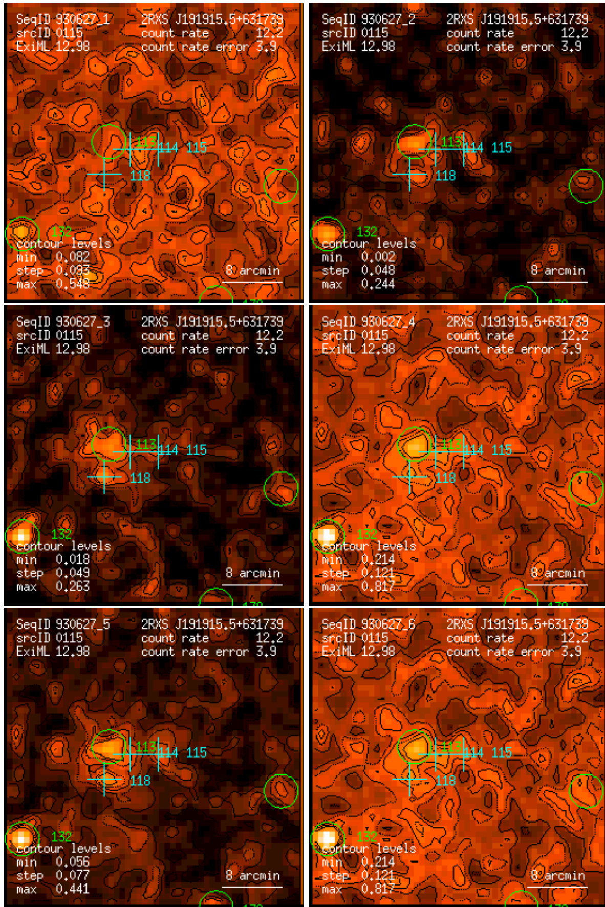
Figure 115: RASS 930627: detection 0115: band rate images, Gaussian filter: (1) PSPC channels 11 – 41, (2) 52 – 90, (3) 91 – 201, (4) 11 – 235, (5) 52 – 201, (6) 11 – 201. Broad band rates in counts/ks. Band rate contour levels in counts/ks/arcmin 2 .
