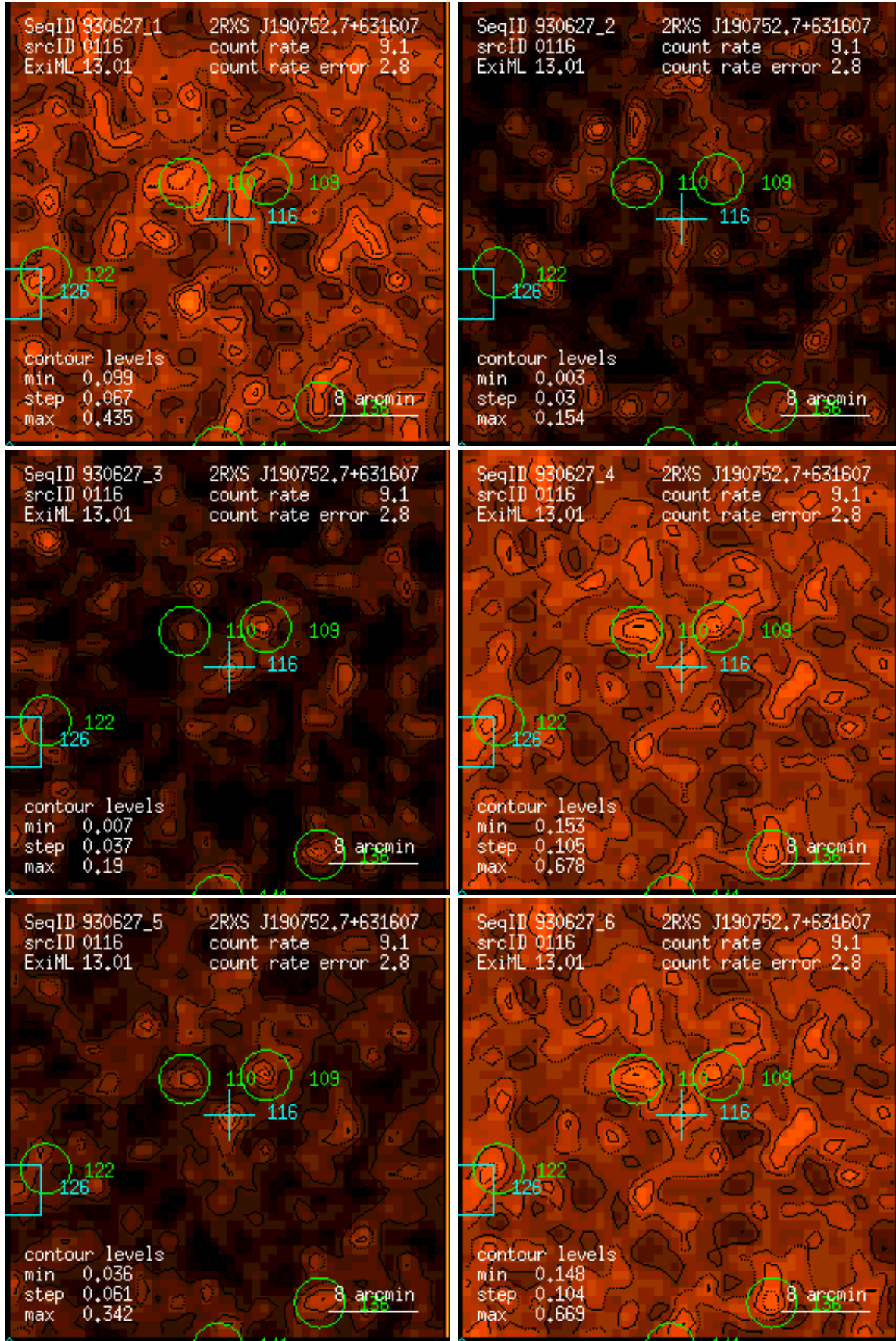
Figure 116: RASS 930627: detection 0116: band rate images, Gaussian filter: (1) PSPC channels 11 – 41, (2) 52 – 90, (3) 91 – 201, (4) 11 – 235, (5) 52 – 201, (6) 11 – 201. Broad band rates in counts/ks. Band rate contour levels in counts/ks/arcmin 2 .
