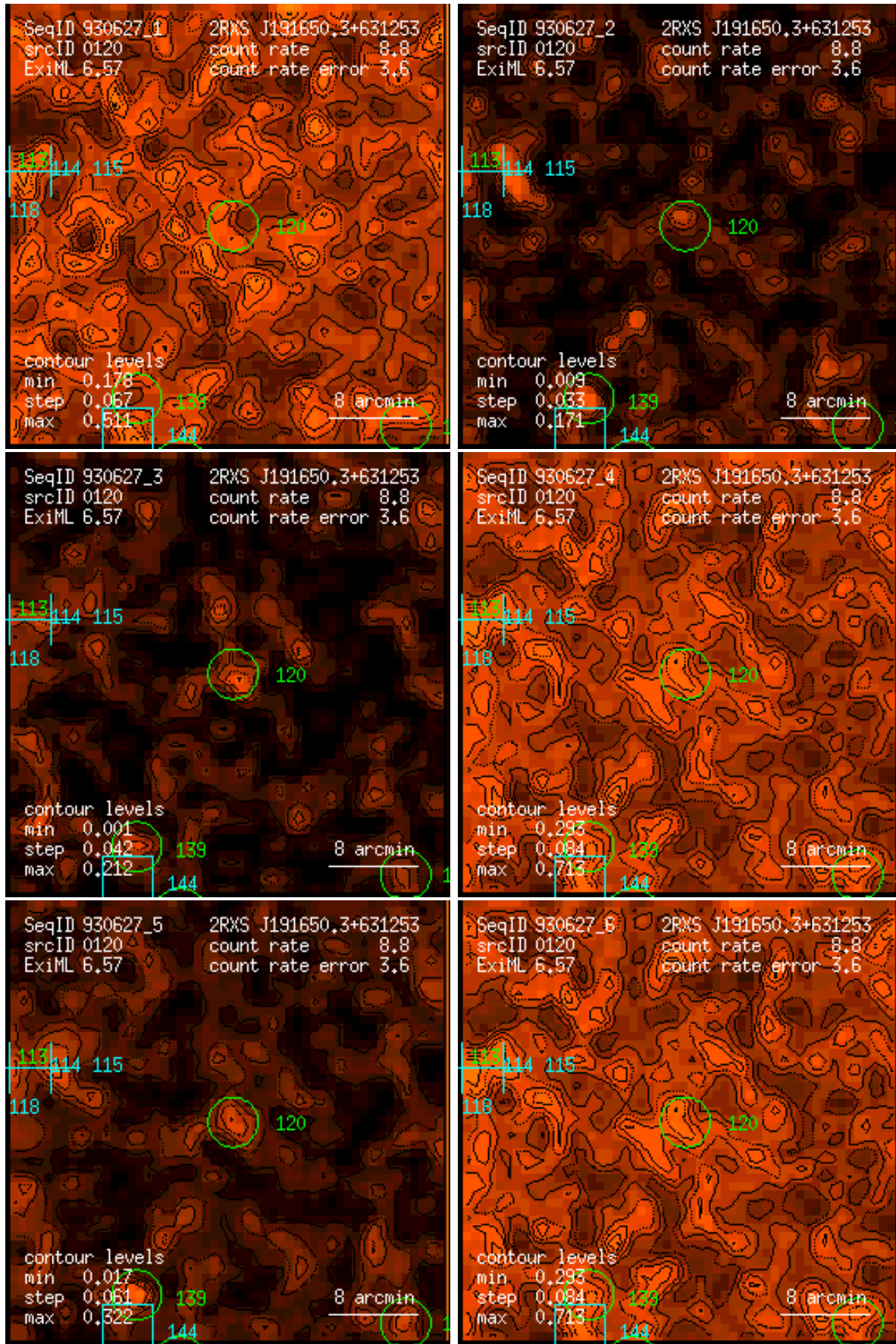
Figure 120: RASS 930627: detection 0120: band rate images, Gaussian filter: (1) PSPC channels 11 – 41, (2) 52 – 90, (3) 91 – 201, (4) 11 – 235, (5) 52 – 201, (6) 11 – 201. Broad band rates in counts/ks. Band rate contour levels in counts/ks/arcmin 2 .
