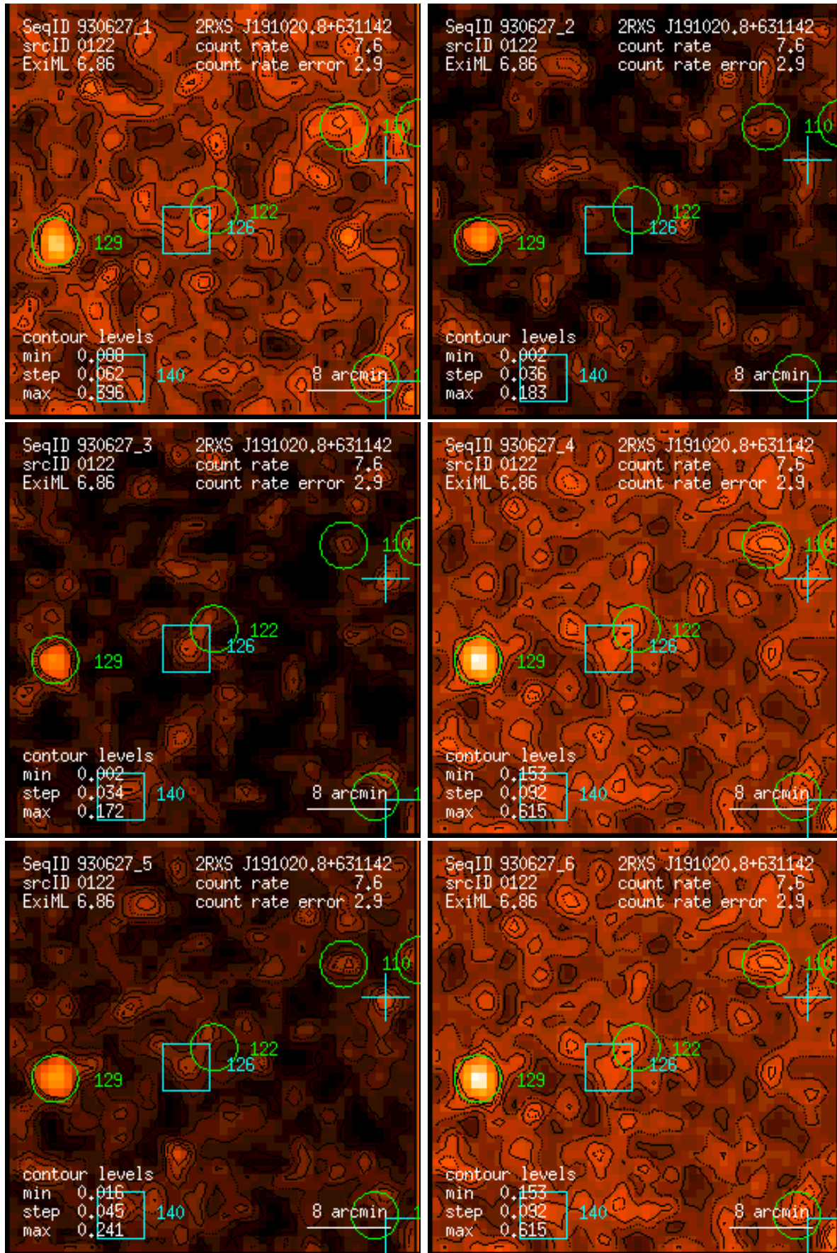
Figure 122: RASS 930627: detection 0122: band rate images, Gaussian filter: (1) PSPC channels 11 – 41, (2) 52 – 90, (3) 91 – 201, (4) 11 – 235, (5) 52 – 201, (6) 11 – 201. Broad band rates in counts/ks. Band rate contour levels in counts/ks/arcmin 2 .
