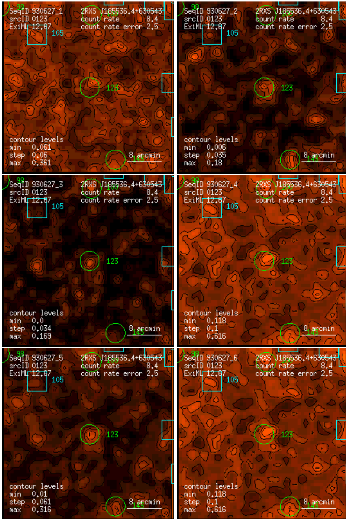
Figure 123: RASS 930627: detection 0123: band rate images, Gaussian filter: (1) PSPC channels 11 – 41, (2) 52 – 90, (3) 91 – 201, (4) 11 – 235, (5) 52 – 201, (6) 11 – 201. Broad band rates in counts/ks. Band rate contour levels in counts/ks/arcmin 2 .
