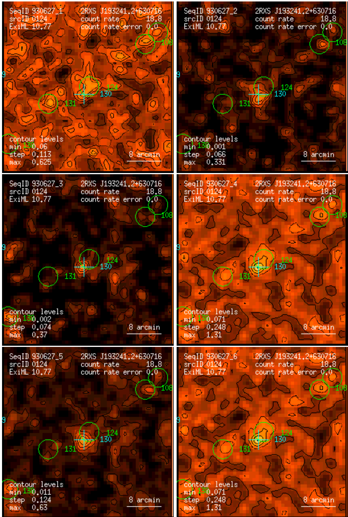
Figure 124: RASS 930627: detection 0124: band rate images, Gaussian filter: (1) PSPC channels 11 – 41, (2) 52 – 90, (3) 91 – 201, (4) 11 – 235, (5) 52 – 201, (6) 11 – 201. Broad band rates in counts/ks. Band rate contour levels in counts/ks/arcmin 2 .
