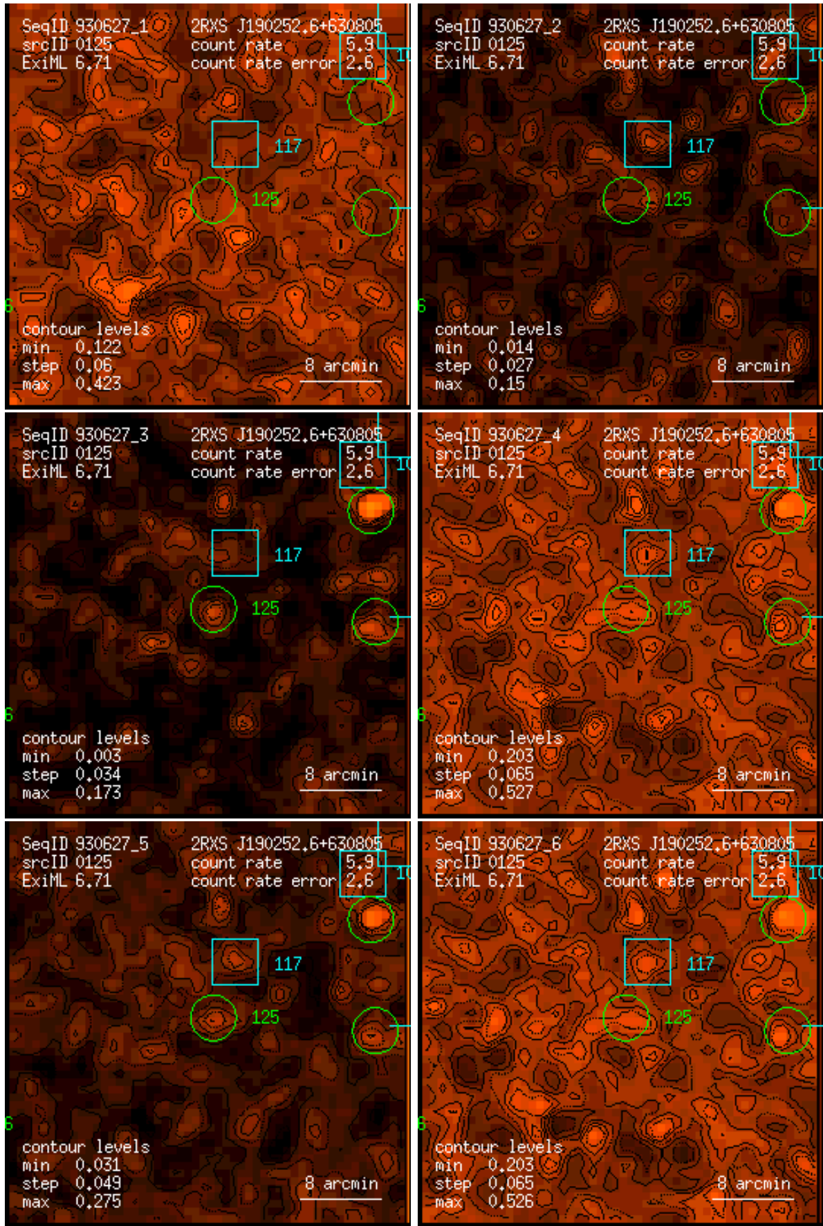
Figure 125: RASS 930627: detection 0125: band rate images, Gaussian filter: (1) PSPC channels 11 – 41, (2) 52 – 90, (3) 91 – 201, (4) 11 – 235, (5) 52 – 201, (6) 11 – 201. Broad band rates in counts/ks. Band rate contour levels in counts/ks/arcmin 2 .
