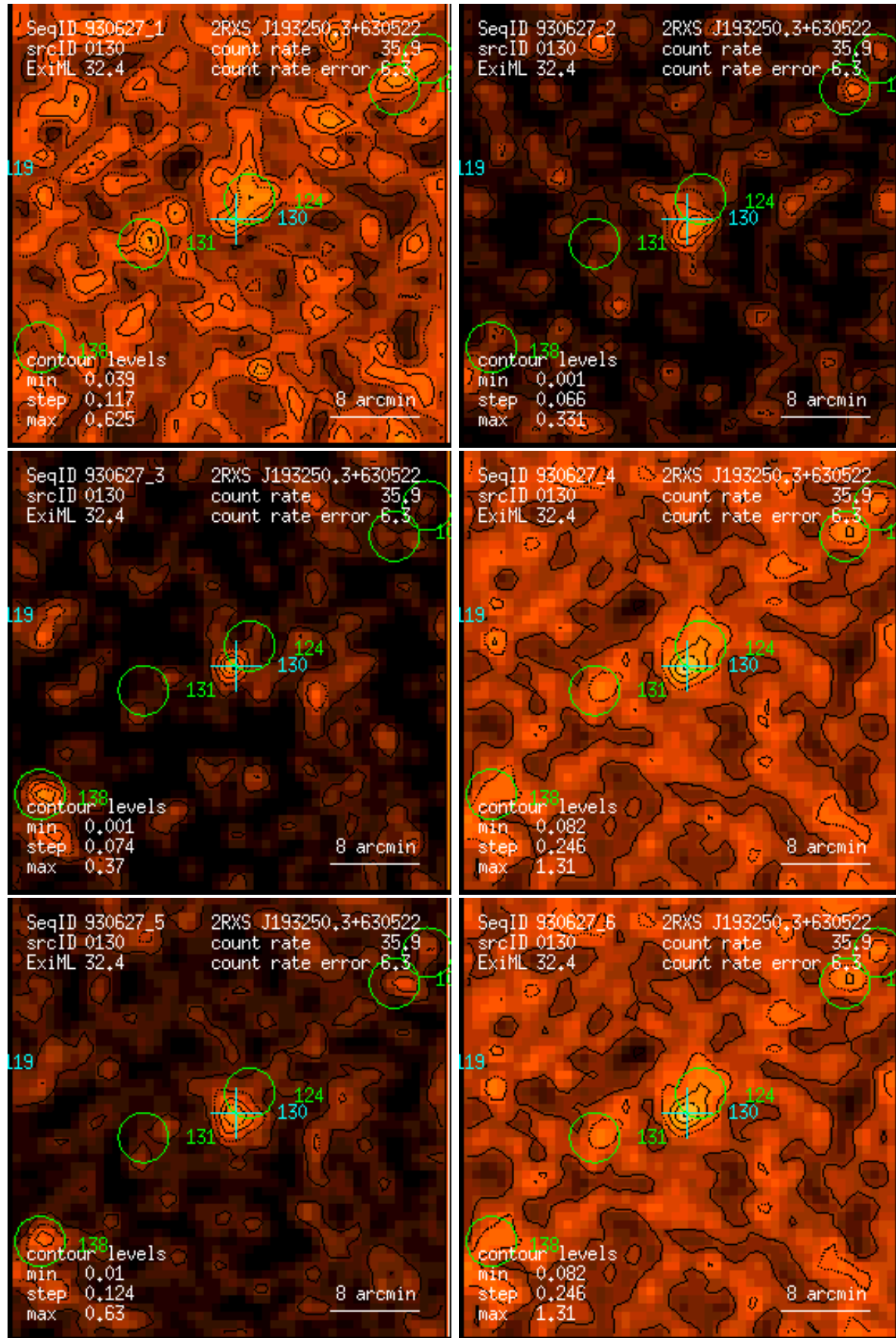
Figure 130: RASS 930627: detection 0130: band rate images, Gaussian filter: (1) PSPC channels 11 – 41, (2) 52 – 90, (3) 91 – 201, (4) 11 – 235, (5) 52 – 201, (6) 11 – 201. Broad band rates in counts/ks. Band rate contour levels in counts/ks/arcmin 2 .
