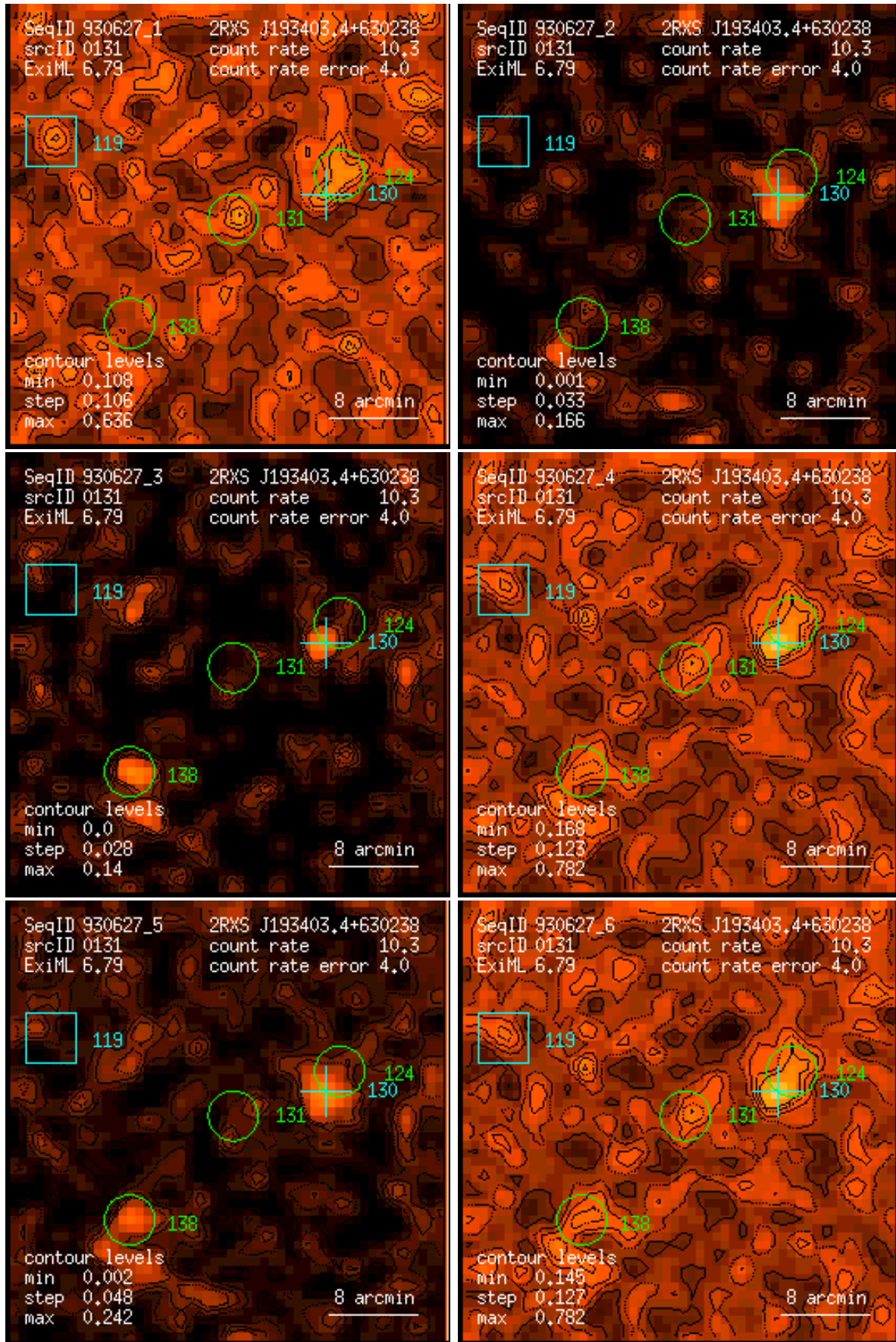
Figure 131: RASS 930627: detection 0131: band rate images, Gaussian filter: (1) PSPC channels 11 – 41, (2) 52 – 90, (3) 91 – 201, (4) 11 – 235, (5) 52 – 201, (6) 11 – 201. Broad band rates in counts/ks. Band rate contour levels in counts/ks/arcmin 2 .
