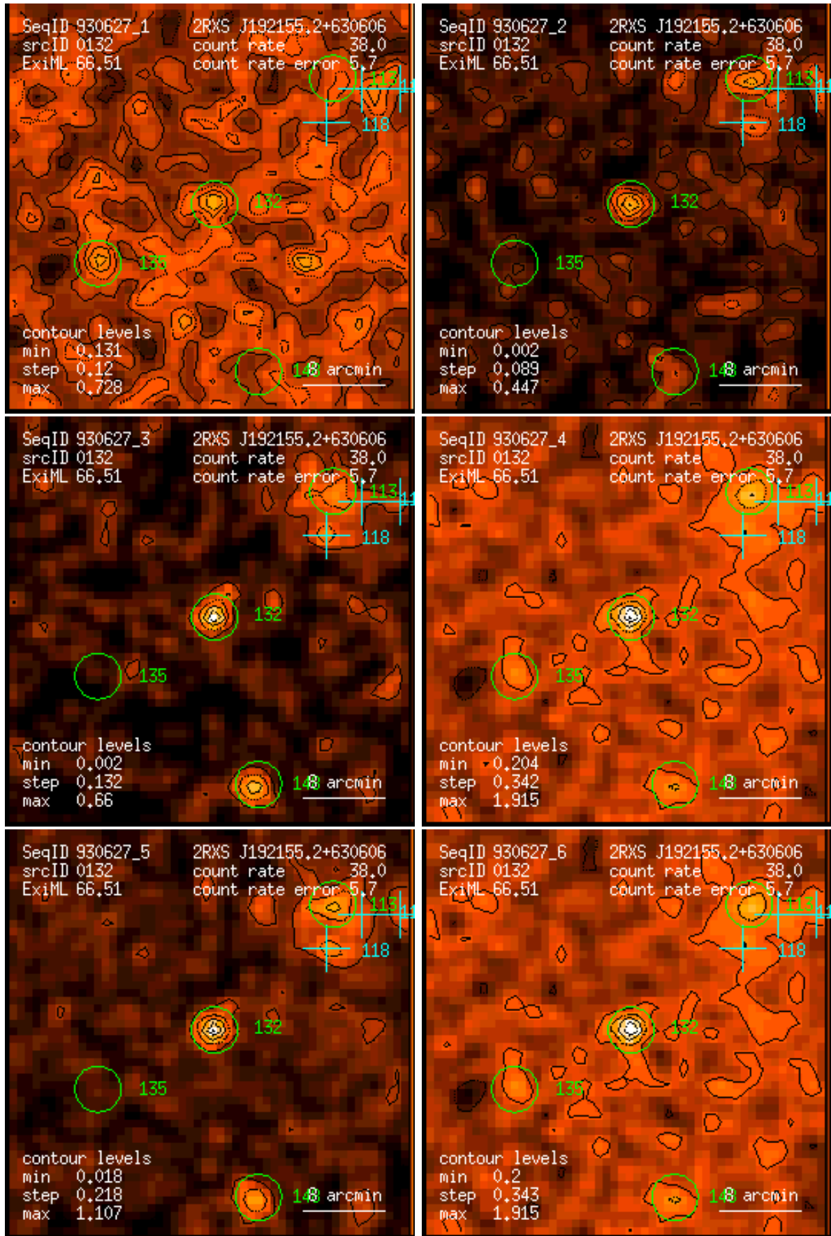
Figure 132: RASS 930627: detection 0132: band rate images, Gaussian filter: (1) PSPC channels 11 – 41, (2) 52 – 90, (3) 91 – 201, (4) 11 – 235, (5) 52 – 201, (6) 11 – 201. Broad band rates in counts/ks. Band rate contour levels in counts/ks/arcmin 2 .
