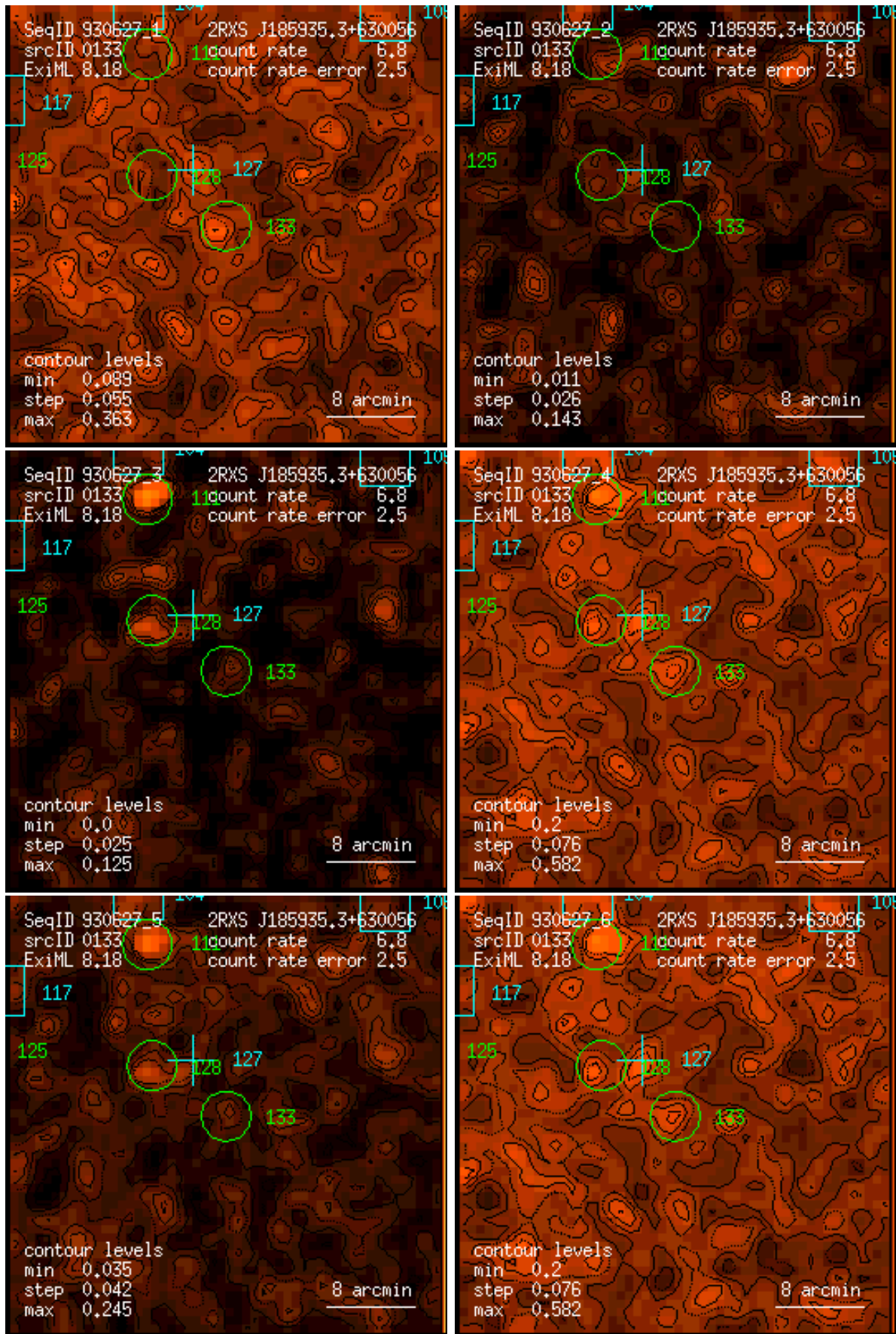
Figure 133: RASS 930627: detection 0133: band rate images, Gaussian filter: (1) PSPC channels 11 – 41, (2) 52 – 90, (3) 91 – 201, (4) 11 – 235, (5) 52 – 201, (6) 11 – 201. Broad band rates in counts/ks. Band rate contour levels in counts/ks/arcmin 2 .
