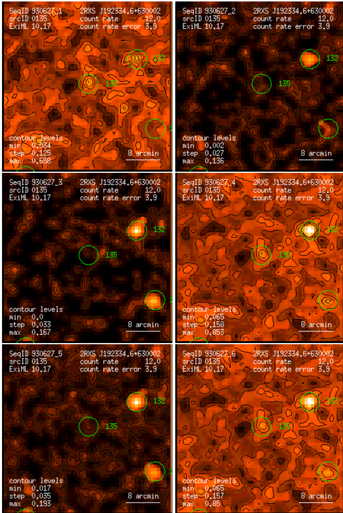
Figure 135: RASS 930627: detection 0135: band rate images, Gaussian filter: (1) PSPPC channels 11 – 41, (2) 52 – 90, (3) 91 – 201, (4) 11 – 235, (5) 52 – 201, (6) 11 – 201. Broad band rates in counts/ks. Band rate contour levels in counts/ks/arcmin 2 .
