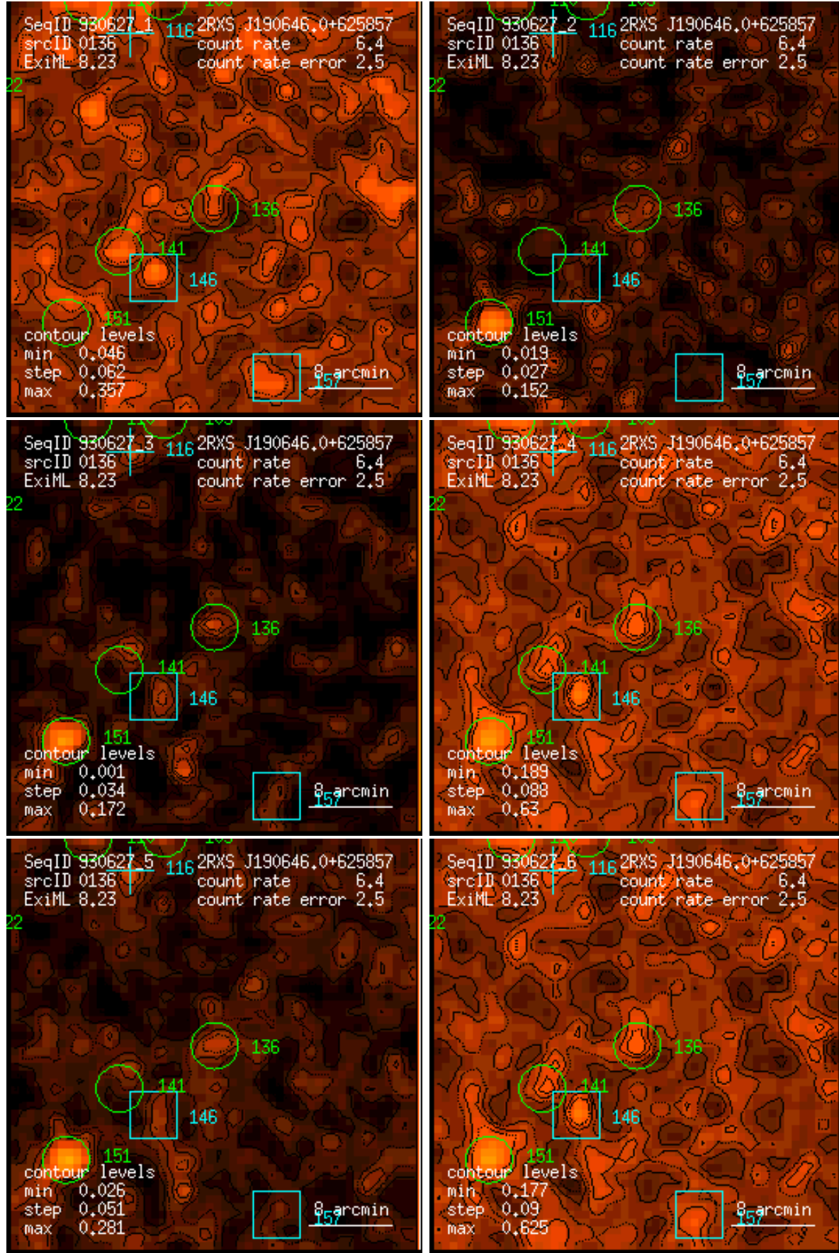
Figure 136: RASS 930627: detection 0136: band rate images, Gaussian filter: (1) PSPC channels 11 – 41, (2) 52 – 90, (3) 91 – 201, (4) 11 – 235, (5) 52 – 201, (6) 11 – 201. Broad band rates in counts/ks. Band rate contour levels in counts/ks/arcmin 2 .
