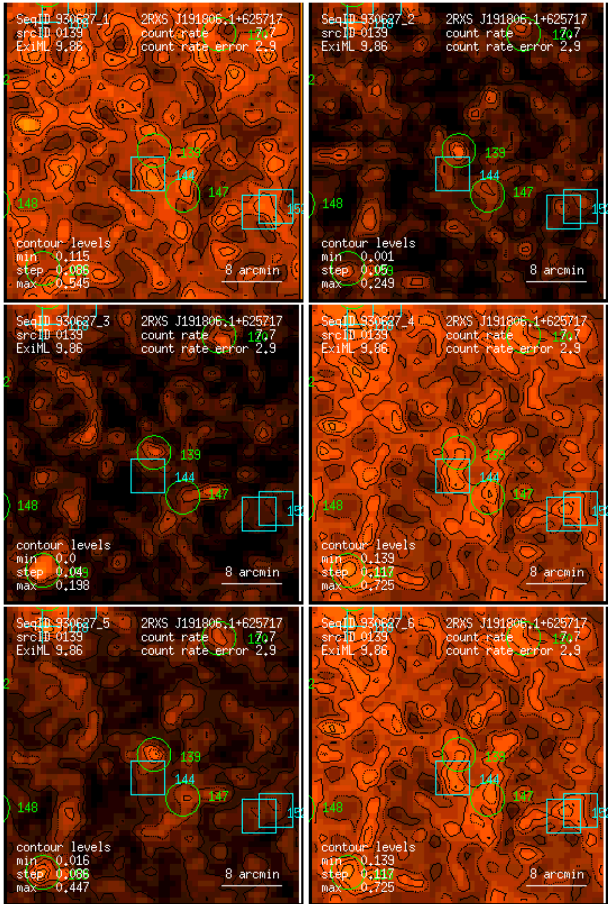
Figure 139: RASS 930627: detection 0139: band rate images, Gaussian filter: (1) PSPC channels 11 – 41, (2) 52 – 90, (3) 91 – 201, (4) 11 – 235, (5) 52 – 201, (6) 11 – 201. Broad band rates in counts/ks. Band rate contour levels in counts/ks/arcmin 2 .
