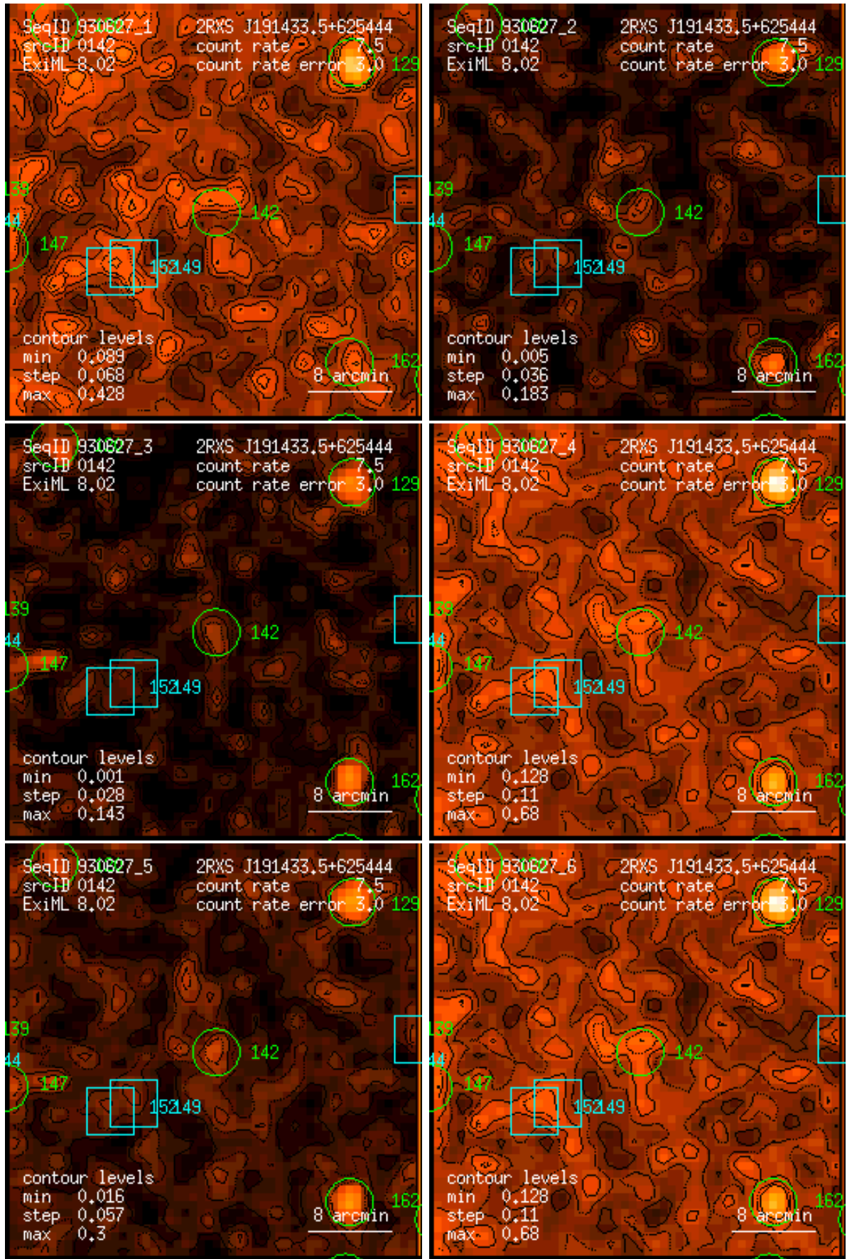
Figure 142: RASS 930627: detection 0142: band rate images, Gaussian filter: (1) PSPC channels 11 – 41, (2) 52 – 90, (3) 91 – 201, (4) 11 – 235, (5) 52 – 201, (6) 11 – 201. Broad band rates in counts/ks. Band rate contour levels in counts/ks/arcmin 2 .
