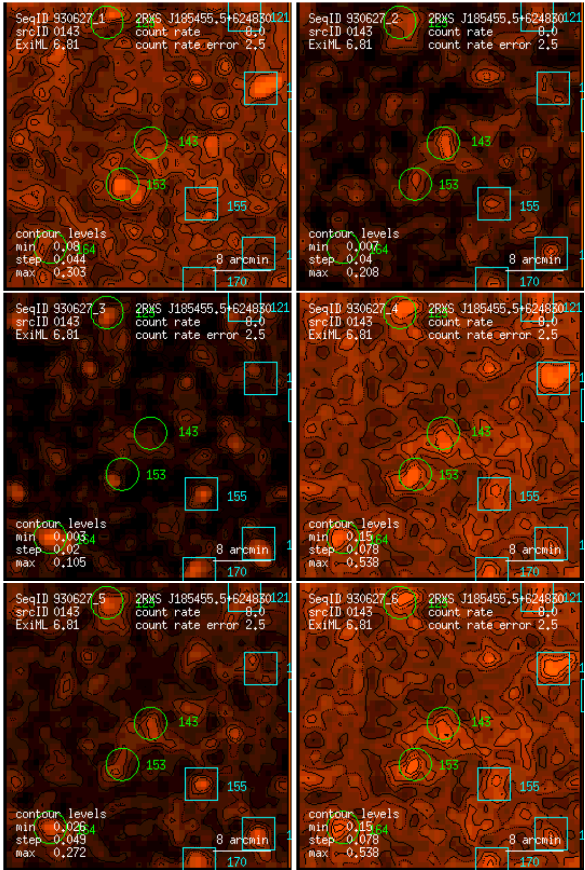
Figure 143: RASS 930627: detection 0143: band rate images, Gaussian filter: (1) PSPC channels 11 – 41, (2) 52 – 90, (3) 91 – 201, (4) 11 – 235, (5) 52 – 201, (6) 11 – 201. Broad band rates in counts/ks. Band rate contour levels in counts/ks/arcmin 2 .
