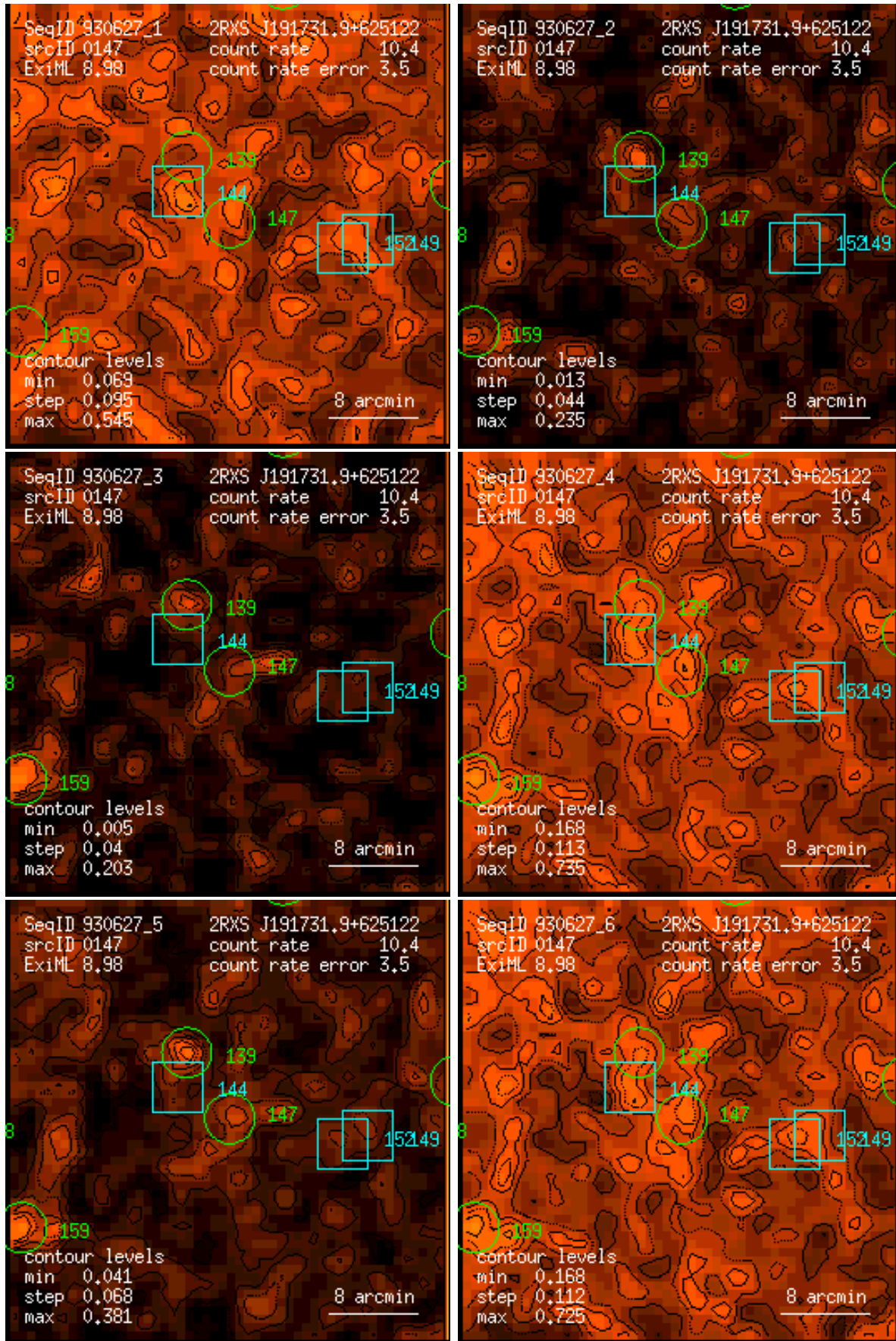
Figure 147: RASS 930627: detection 0147: band rate images, Gaussian filter: (1) PSPC channels 11 – 41, (2) 52 – 90, (3) 91 – 201, (4) 11 – 235, (5) 52 – 201, (6) 11 – 201. Broad band rates in counts/ks. Band rate contour levels in counts/ks/arcmin 2 .
